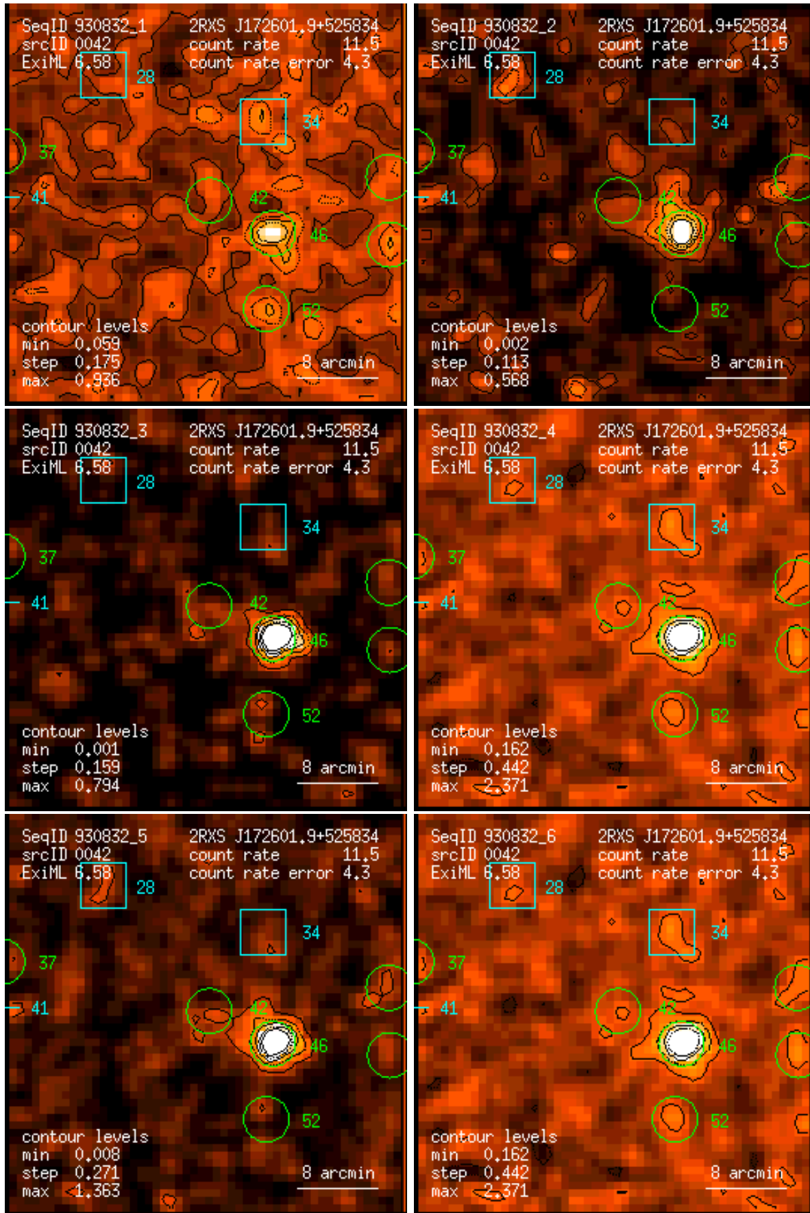
Figure 42: RASS 930832: detection 0042: band rate images, Gaussian filter: (1) PSPC channels 11 – 41, (2) 52 – 90, (3) 91 – 201, (4) 11 – 235, (5) 52 – 201, (6) 11 – 201. Broad band rates in counts/ks. Band rate contour levels in counts/ks/arcmin 2 .
