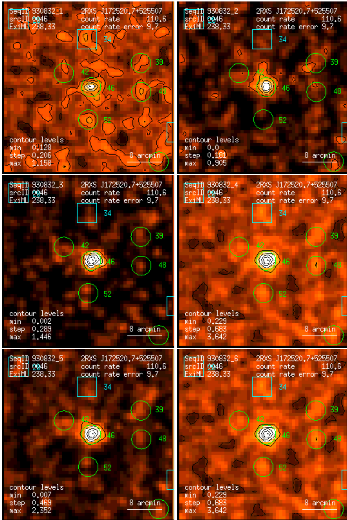
Figure 46: RASS 930832: detection 0046: band rate images, Gaussian filter: (1) PSPC channels 11 – 41, (2) 52 – 90, (3) 91 – 201, (4) 11 – 235, (5) 52 – 201, (6) 11 – 201. Broad band rates in counts/ks. Band rate contour levels in counts/ks/arcmin 2 .
