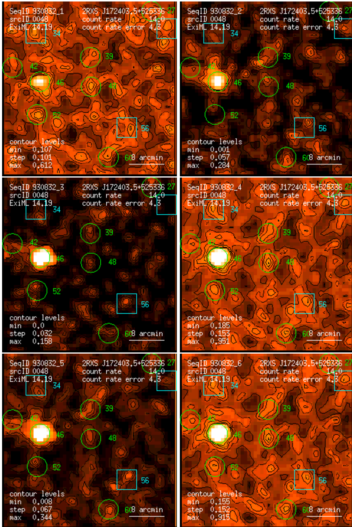
Figure 48: RASS 930832: detection 0048: band rate images, Gaussian filter: (1) PSPC channels 11 – 41, (2) 52 – 90, (3) 91 – 201, (4) 11 – 235, (5) 52 – 201, (6) 11 – 201. Broad band rates in counts/ks. Band rate contour levels in counts/ks/arcmin 2 .
