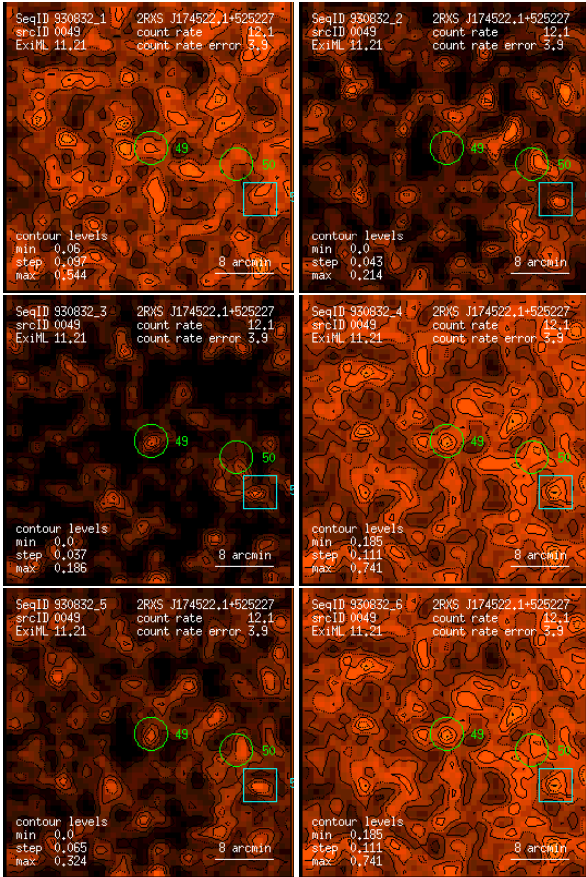
Figure 49: RASS 930832: detection 0049: band rate images, Gaussian filter: (1) PSPC channels 11 – 41, (2) 52 – 90, (3) 91 – 201, (4) 11 – 235, (5) 52 – 201, (6) 11 – 201. Broad band rates in counts/ks. Band rate contour levels in counts/ks/arcmin 2 .
