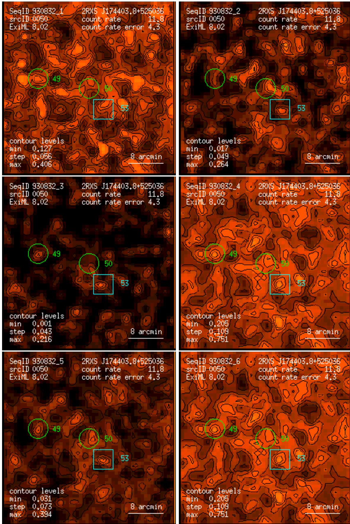
Figure 50: RASS 930832: detection 0050: band rate images, Gaussian filter: (1) PSPC channels 11 – 41, (2) 52 – 90, (3) 91 – 201, (4) 11 – 235, (5) 52 – 201, (6) 11 – 201. Broad band rates in counts/ks. Band rate contour levels in counts/ks/arcmin 2 .
