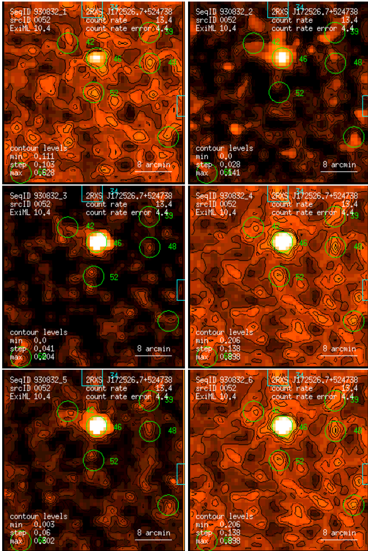
Figure 52: RASS 930832: detection 0052: band rate images, Gaussian filter: (1) PSPC channels 11 – 41, (2) 52 – 90, (3) 91 – 201, (4) 11 – 235, (5) 52 – 201, (6) 11 – 201. Broad band rates in counts/ks. Band rate contour levels in counts/ks/arcmin 2 .
