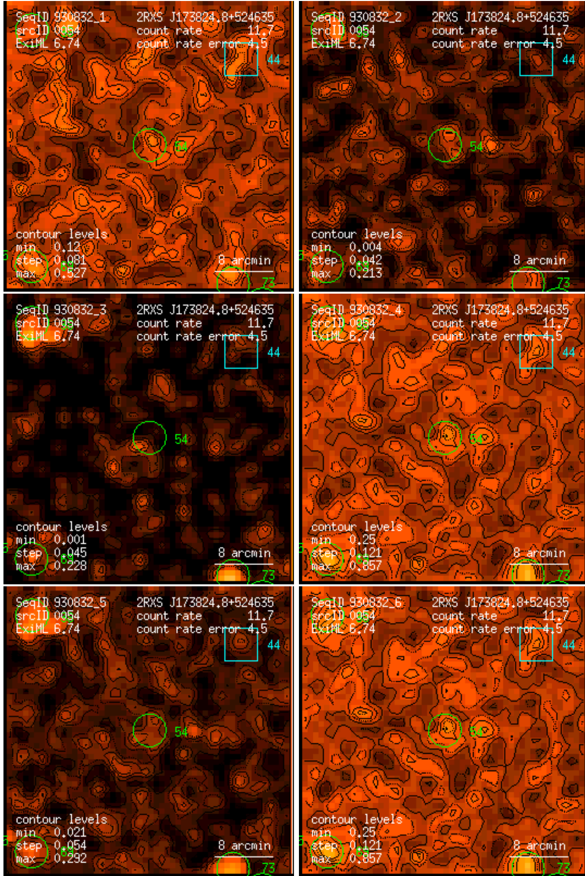
Figure 54: RASS 930832: detection 0054: band rate images, Gaussian filter: (1) PSPC channels 11 – 41, (2) 52 – 90, (3) 91 – 201, (4) 11 – 235, (5) 52 – 201, (6) 11 – 201. Broad band rates in counts/ks. Band rate contour levels in counts/ks/arcmin 2 .
