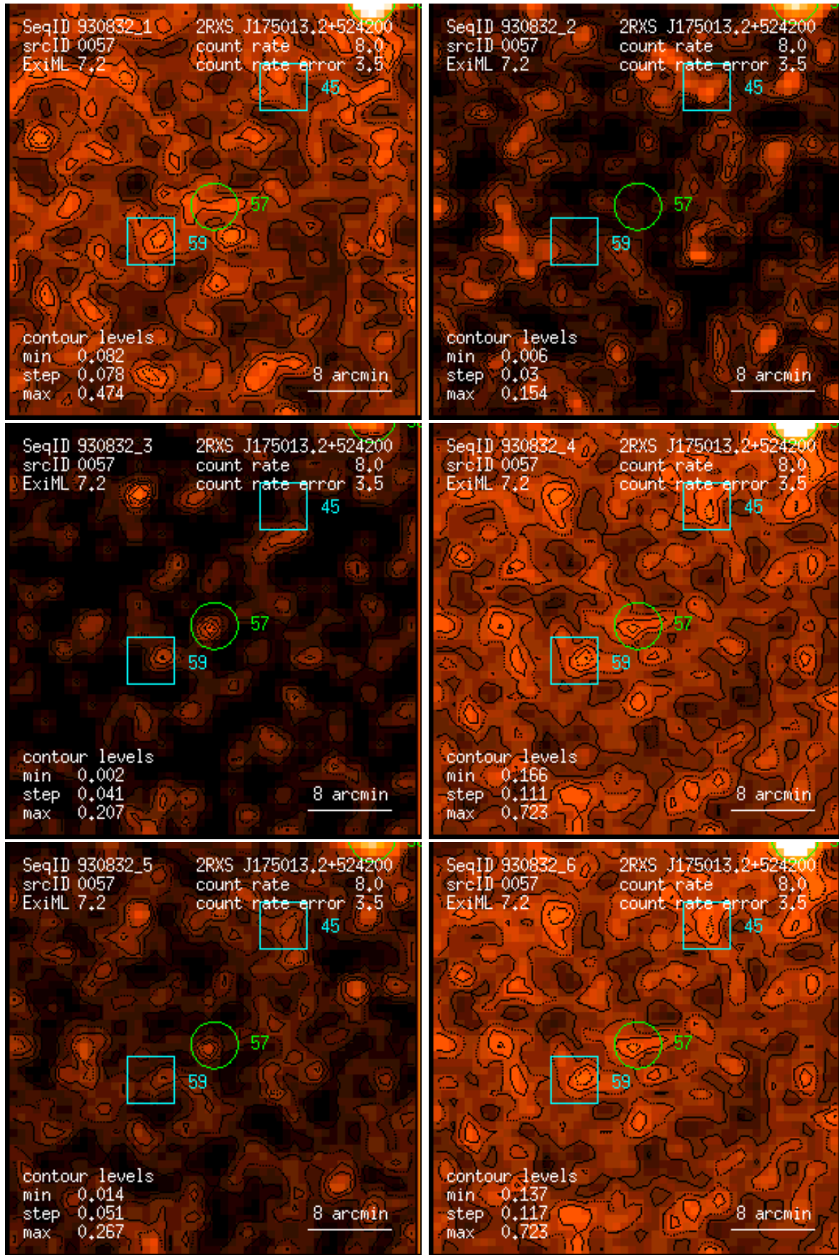
Figure 57: RASS 930832: detection 0057: band rate images, Gaussian filter: (1) PSPC channels 11 – 41, (2) 52 – 90, (3) 91 – 201, (4) 11 – 235, (5) 52 – 201, (6) 11 – 201. Broad band rates in counts/ks. Band rate contour levels in counts/ks/arcmin 2 .
