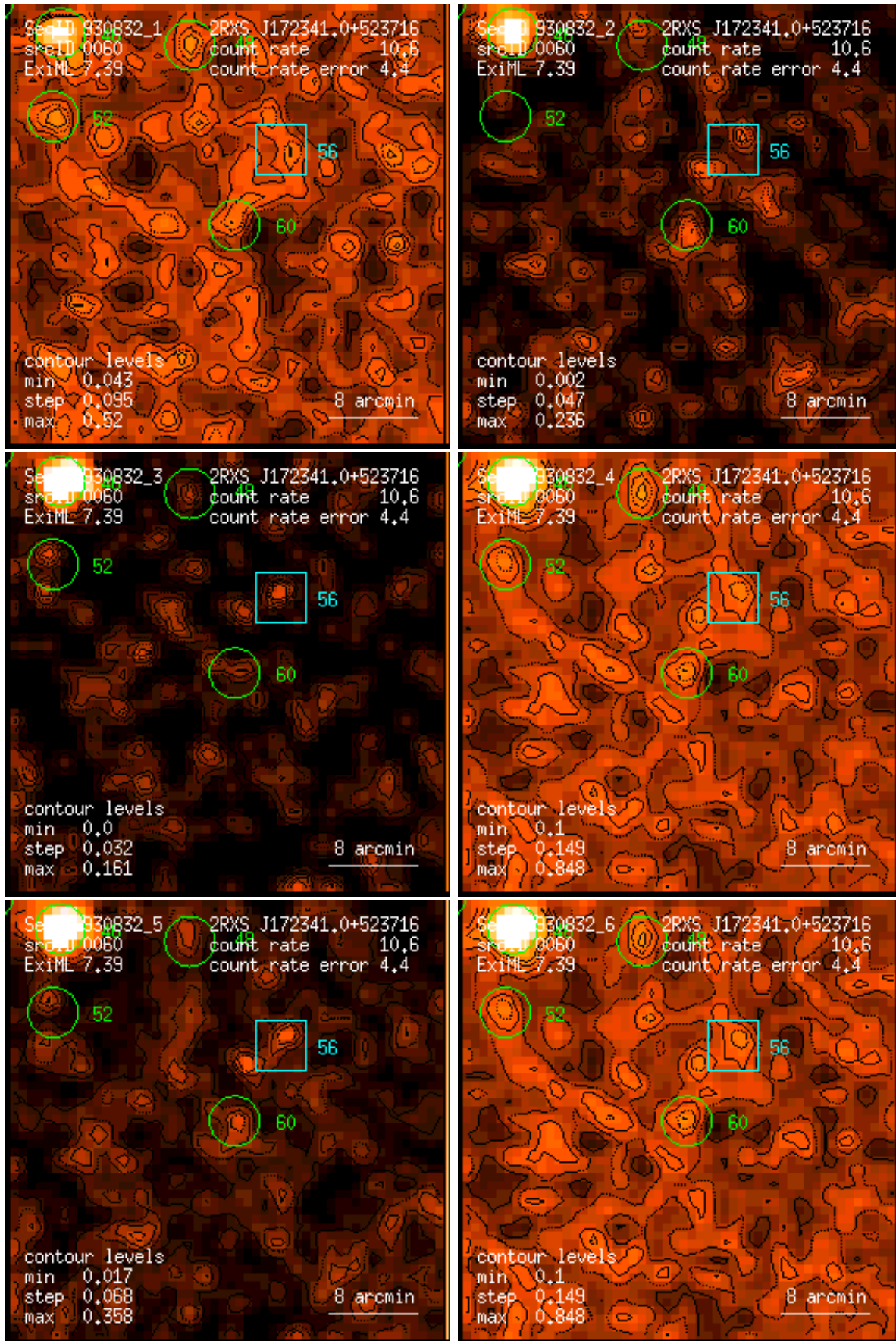
Figure 60: RASS 930832: detection 0060: band rate images, Gaussian filter: (1) PSPC channels 11 – 41, (2) 52 – 90, (3) 91 – 201, (4) 11 – 235, (5) 52 – 201, (6) 11 – 201. Broad band rates in counts/ks. Band rate contour levels in counts/ks/arcmin 2 .
