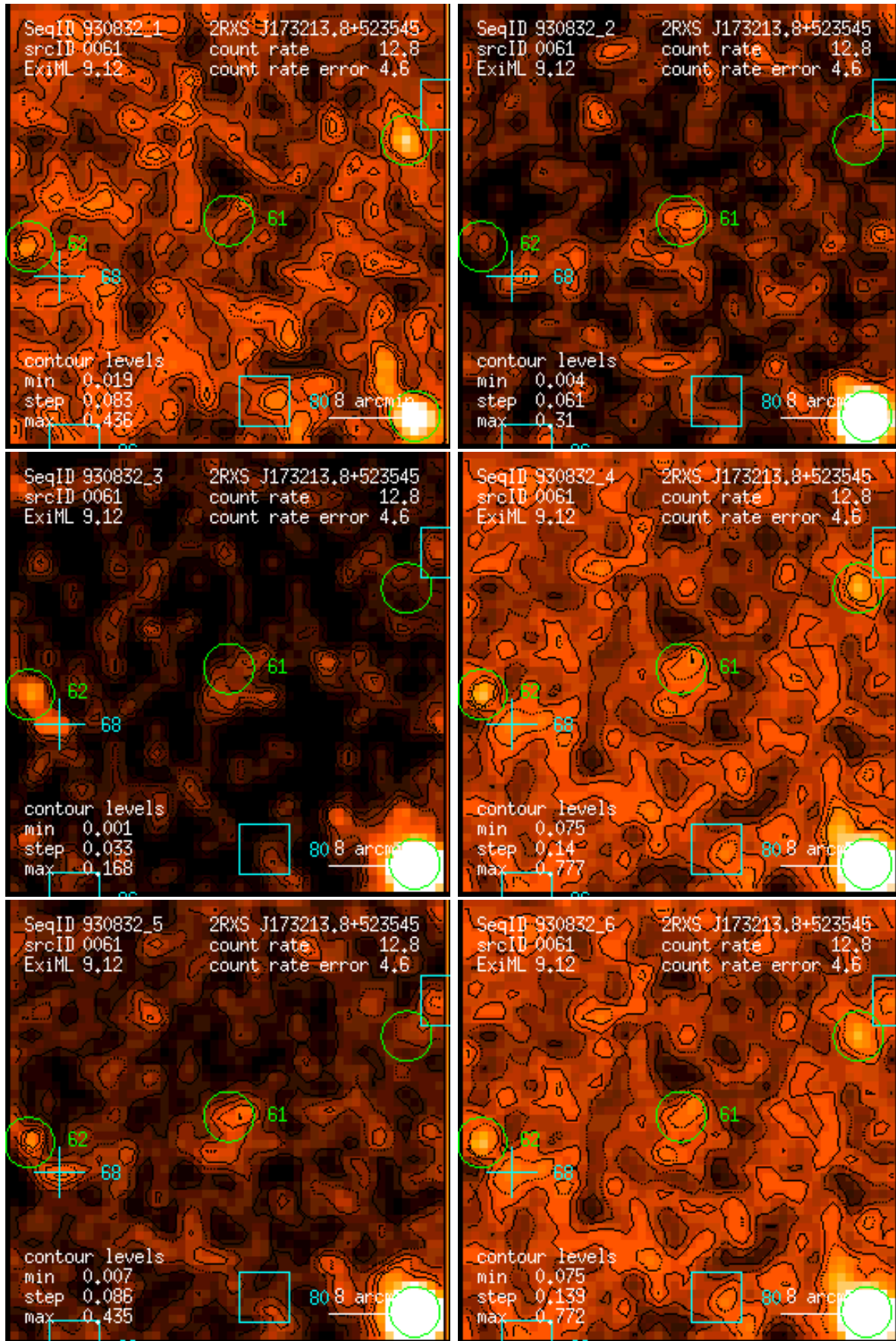
Figure 61: RASS 930832: detection 0061: band rate images, Gaussian filter: (1) PSPC channels 11 – 41, (2) 52 – 90, (3) 91 – 201, (4) 11 – 235, (5) 52 – 201, (6) 11 – 201. Broad band rates in counts/ks. Band rate contour levels in counts/ks/arcmin 2 .
