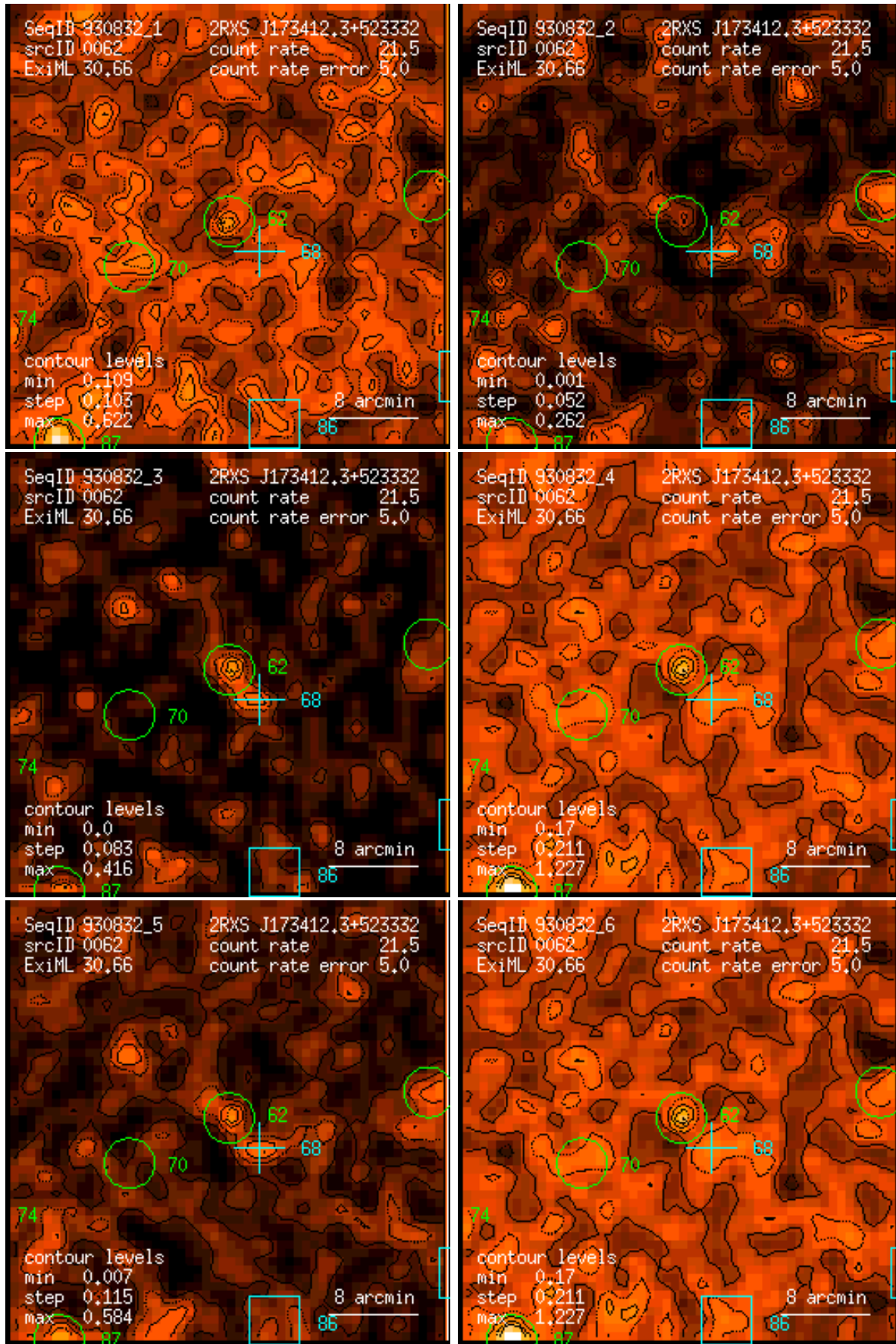
Figure 62: RASS 930832: detection 0062: band rate images, Gaussian filter: (1) PSPC channels 11 – 41, (2) 52 – 90, (3) 91 – 201, (4) 11 – 235, (5) 52 – 201, (6) 11 – 201. Broad band rates in counts/ks. Band rate contour levels in counts/ks/arcmin 2 .
