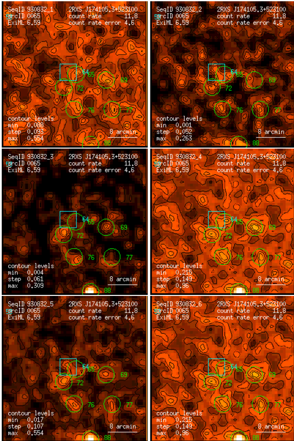
Figure 65: RASS 930832: detection 0065: band rate images, Gaussian filter: (1) PSPC channels 11 – 41, (2) 52 – 90, (3) 91 – 201, (4) 11 – 235, (5) 52 – 201, (6) 11 – 201. Broad band rates in counts/ks. Band rate contour levels in counts/ks/arcmin 2 .
