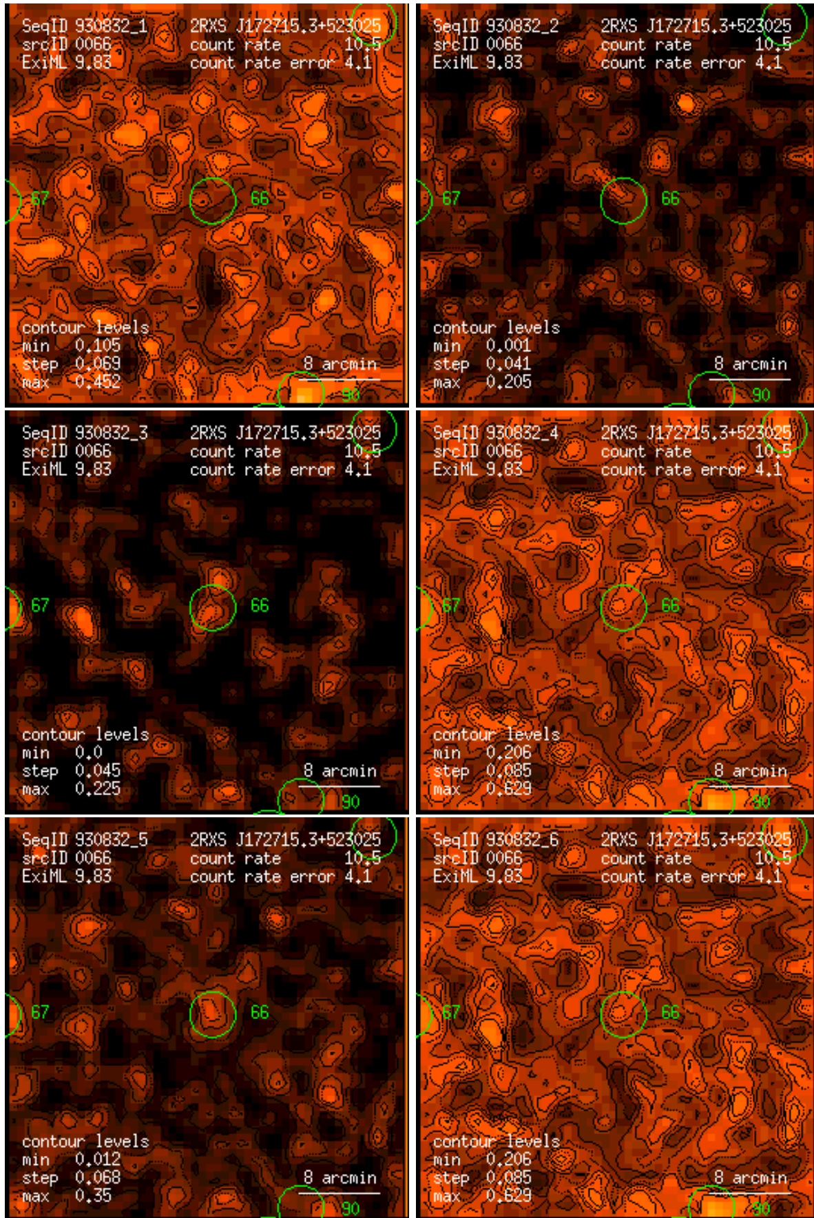
Figure 66: RASS 930832: detection 0066: band rate images, Gaussian filter: (1) PSPC channels 11 – 41, (2) 52 – 90, (3) 91 – 201, (4) 11 – 235, (5) 52 – 201, (6) 11 – 201. Broad band rates in counts/ks. Band rate contour levels in counts/ks/arcmin 2 .
