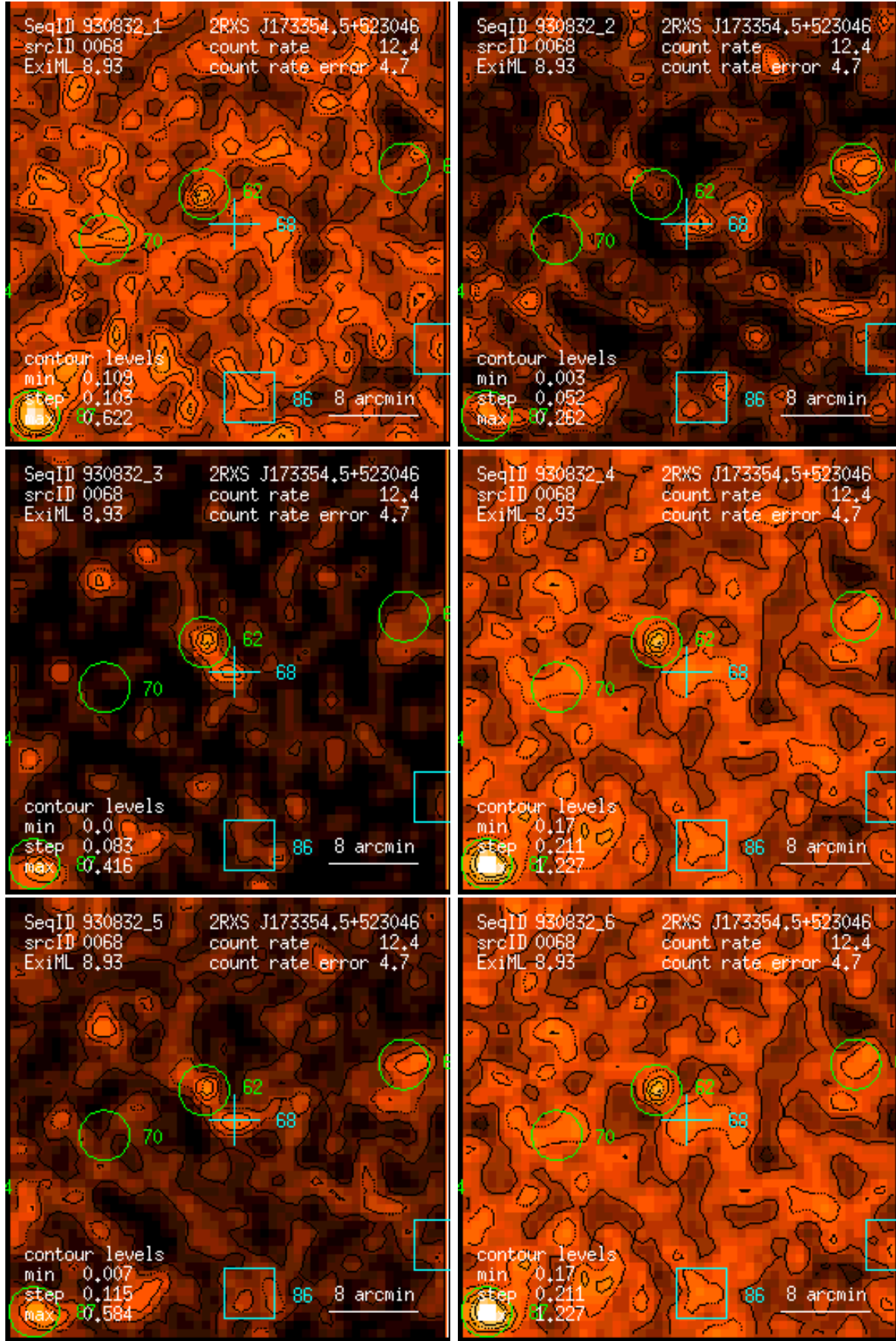
Figure 68: RASS 930832: detection 0068: band rate images, Gaussian filter: (1) PSPC channels 11 – 41, (2) 52 – 90, (3) 91 – 201, (4) 11 – 235, (5) 52 – 201, (6) 11 – 201. Broad band rates in counts/ks. Band rate contour levels in counts/ks/arcmin 2 .
