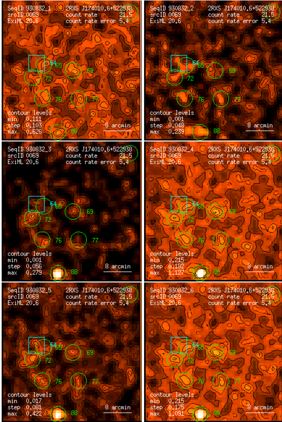
Figure 69: RASS 930832: detection 0069: band rate images, Gaussian filter: (1) PSPC channels 11 – 41, (2) 52 – 90, (3) 91 – 201, (4) 11 – 235, (5) 52 – 201, (6) 11 – 201. Broad band rates in counts/ks. Band rate contour levels in counts/ks/arcmin 2 .
