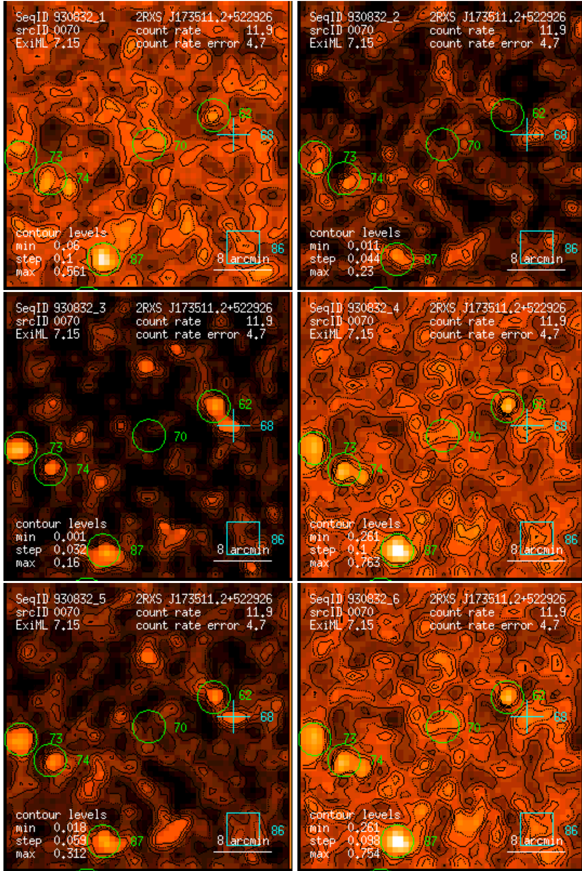
Figure 70: RASS 930832: detection 0070: band rate images, Gaussian filter: (1) PSPC channels 11 – 41, (2) 52 – 90, (3) 91 – 201, (4) 11 – 235, (5) 52 – 201, (6) 11 – 201. Broad band rates in counts/ks. Band rate contour levels in counts/ks/arcmin 2 .
