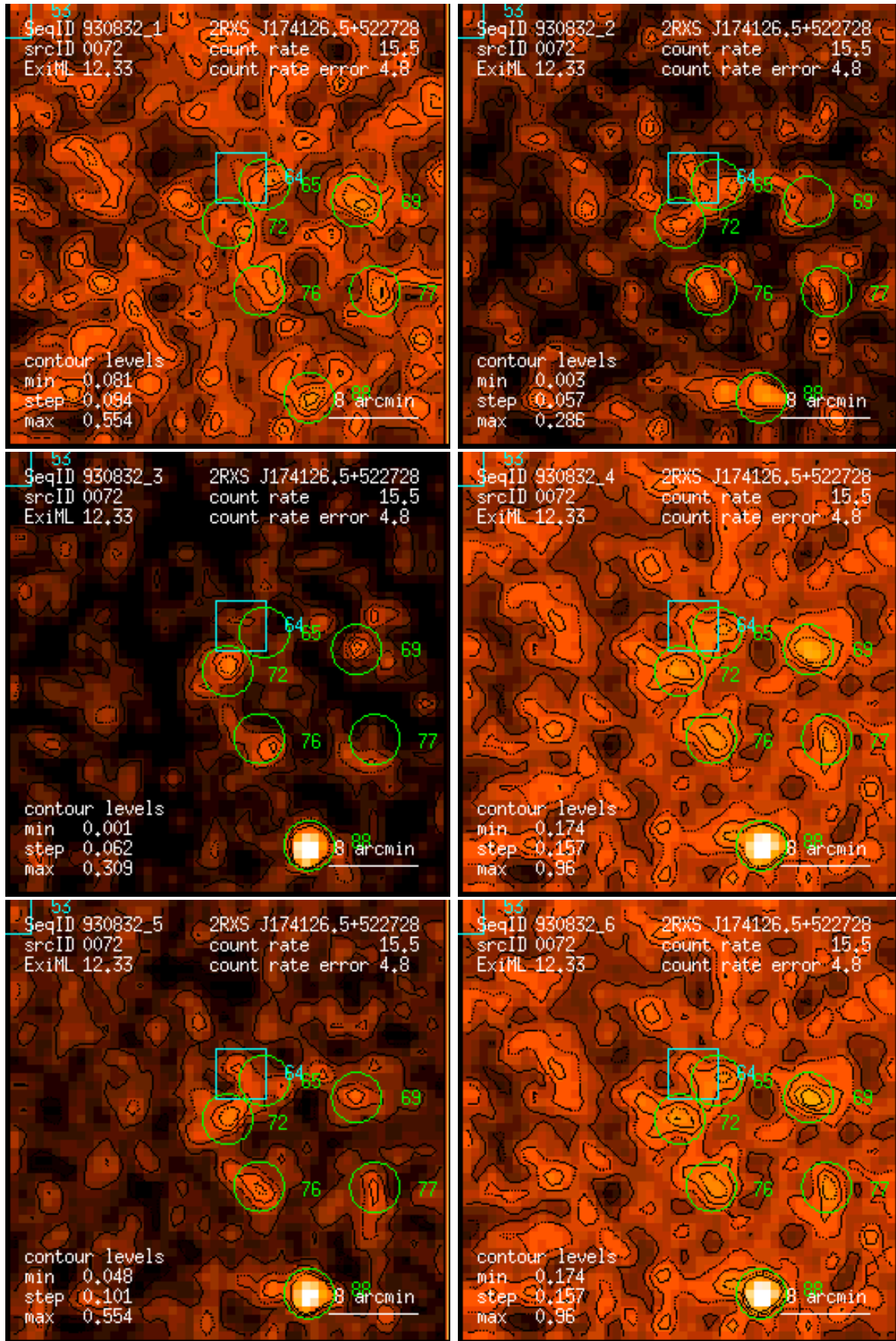
Figure 72: RASS 930832: detection 0072: band rate images, Gaussian filter: (1) PSPC channels 11 – 41, (2) 52 – 90, (3) 91 – 201, (4) 11 – 235, (5) 52 – 201, (6) 11 – 201. Broad band rates in counts/ks. Band rate contour levels in counts/ks/arcmin 2 .
