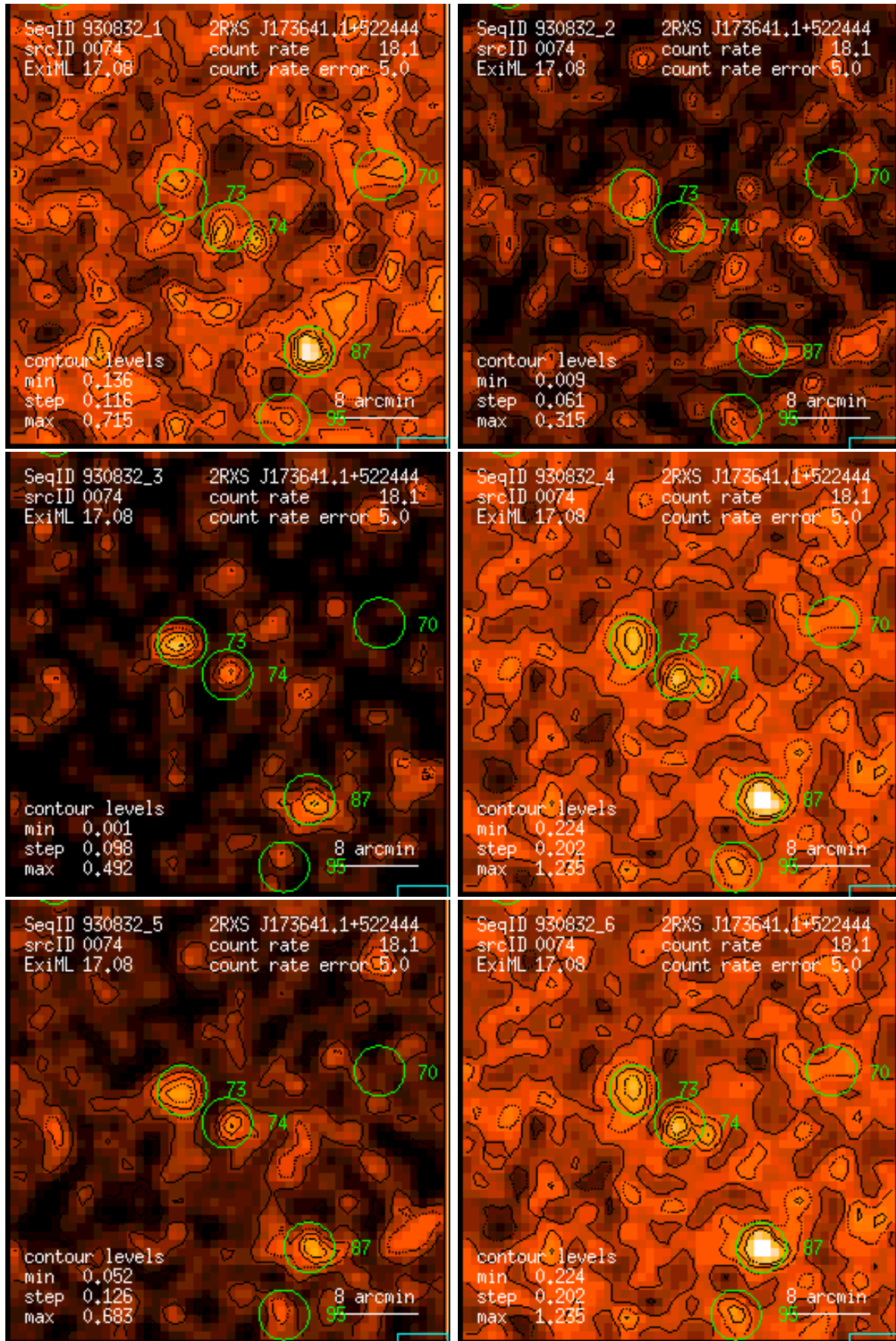
Figure 74: RASS 930832: detection 0074: band rate images, Gaussian filter: (1) PSPC channels 11 – 41, (2) 52 – 90, (3) 91 – 201, (4) 11 – 235, (5) 52 – 201, (6) 11 – 201. Broad band rates in counts/ks. Band rate contour levels in counts/ks/arcmin 2 .
