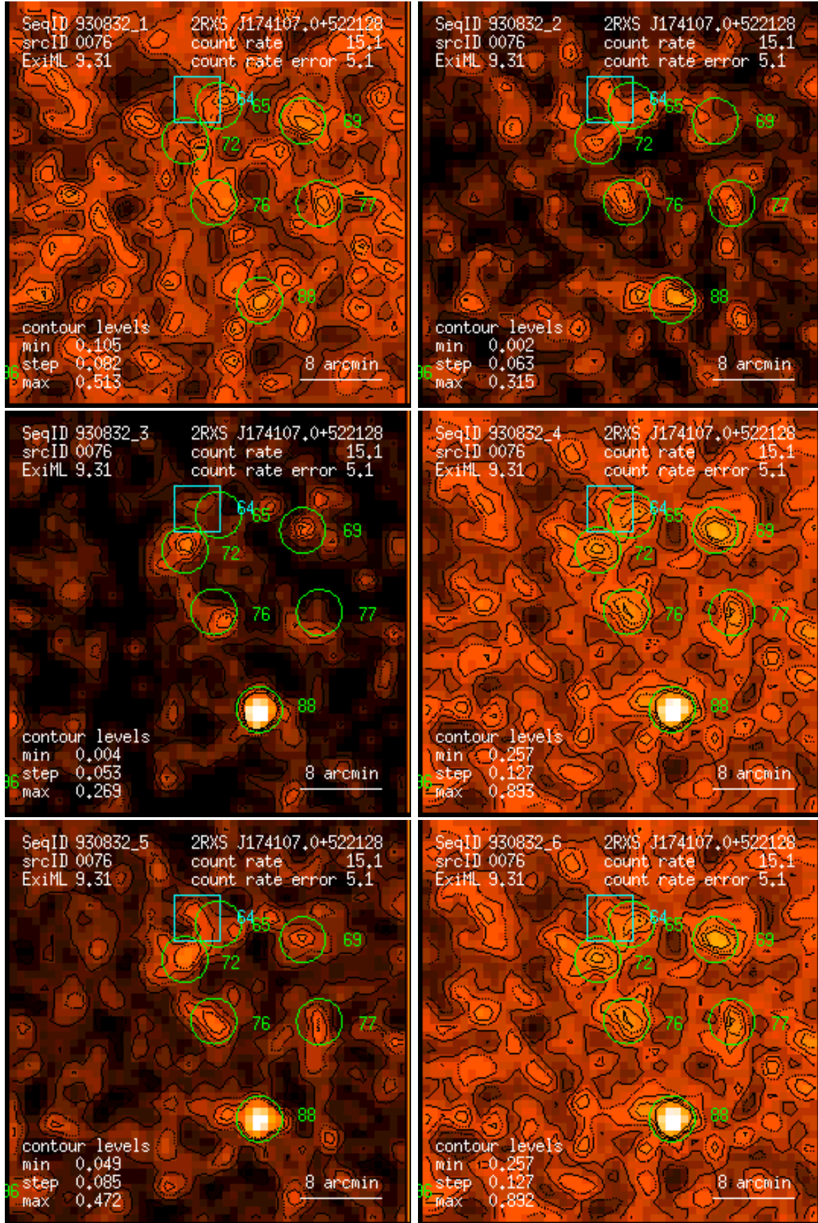
Figure 76: RASS 930832: detection 0076: band rate images, Gaussian filter: (1) PSPC channels 11 – 41, (2) 52 – 90, (3) 91 – 201, (4) 11 – 235, (5) 52 – 201, (6) 11 – 201. Broad band rates in counts/ks. Band rate contour levels in counts/ks/arcmin 2 .
