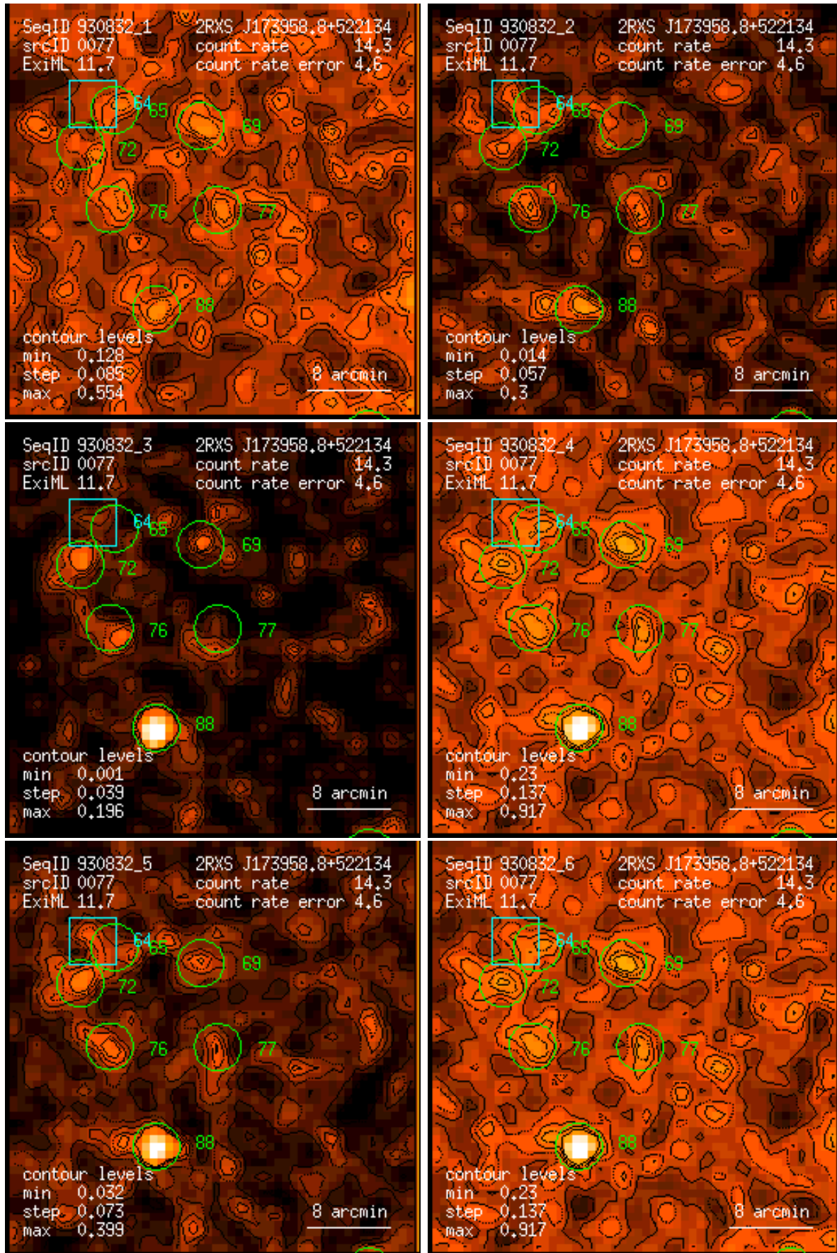
Figure 77: RASS 930832: detection 0077: band rate images, Gaussian filter: (1) PSPC channels 11 – 41, (2) 52 – 90, (3) 91 – 201, (4) 11 – 235, (5) 52 – 201, (6) 11 – 201. Broad band rates in counts/ks. Band rate contour levels in counts/ks/arcmin 2 .
