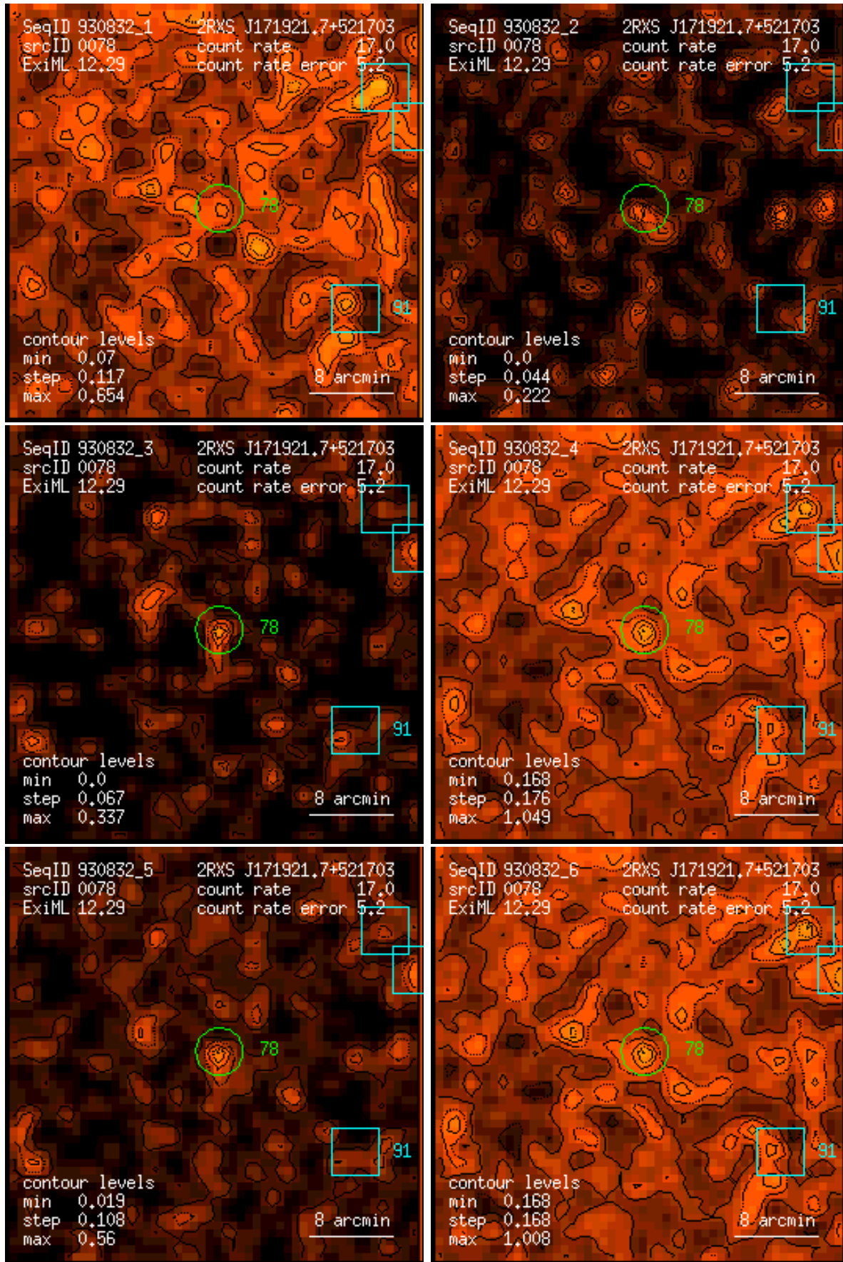
Figure 78: RASS 930832: detection 0078: band rate images, Gaussian filter: (1) PSPC channels 11 – 41, (2) 52 – 90, (3) 91 – 201, (4) 11 – 235, (5) 52 – 201, (6) 11 – 201. Broad band rates in counts/ks. Band rate contour levels in counts/ks/arcmin 2 .
