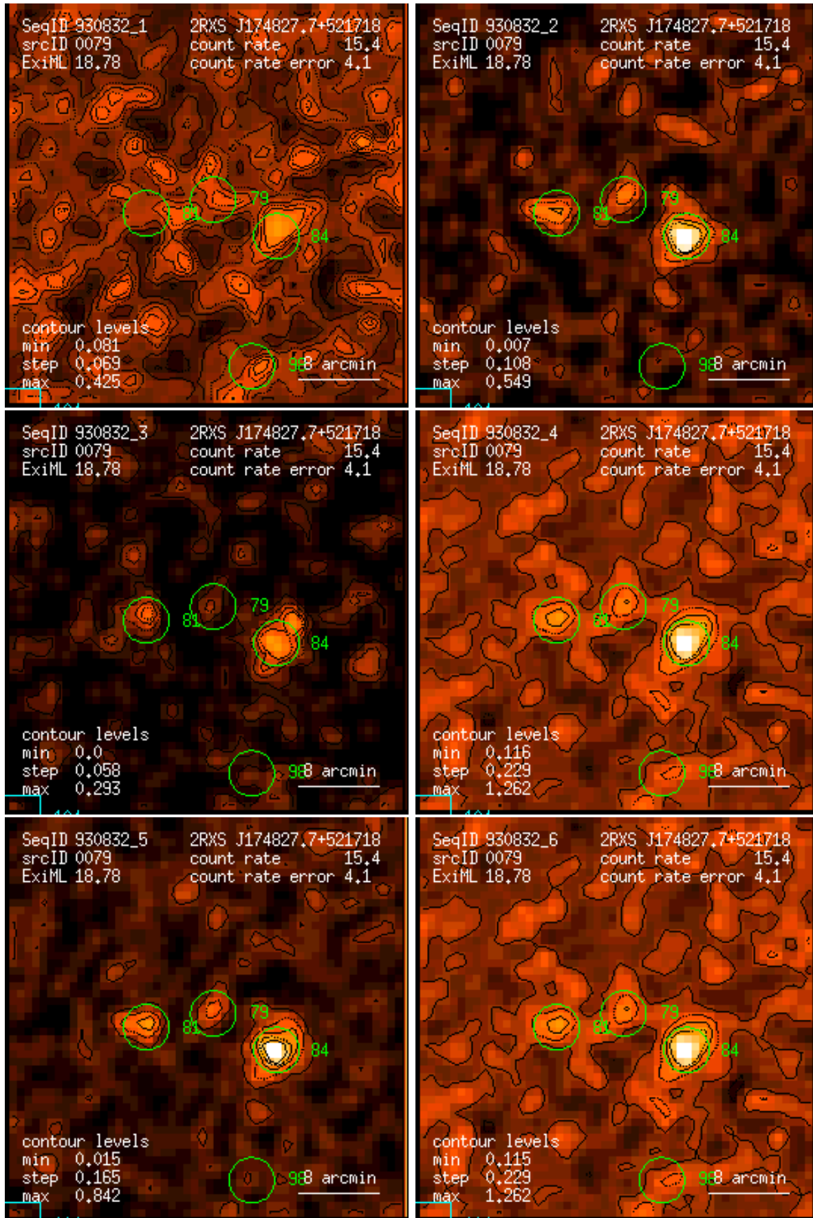
Figure 79: RASS 930832: detection 0079: band rate images, Gaussian filter: (1) PSPC channels 11 – 41, (2) 52 – 90, (3) 91 – 201, (4) 11 – 235, (5) 52 – 201, (6) 11 – 201. Broad band rates in counts/ks. Band rate contour levels in counts/ks/arcmin 2 .
