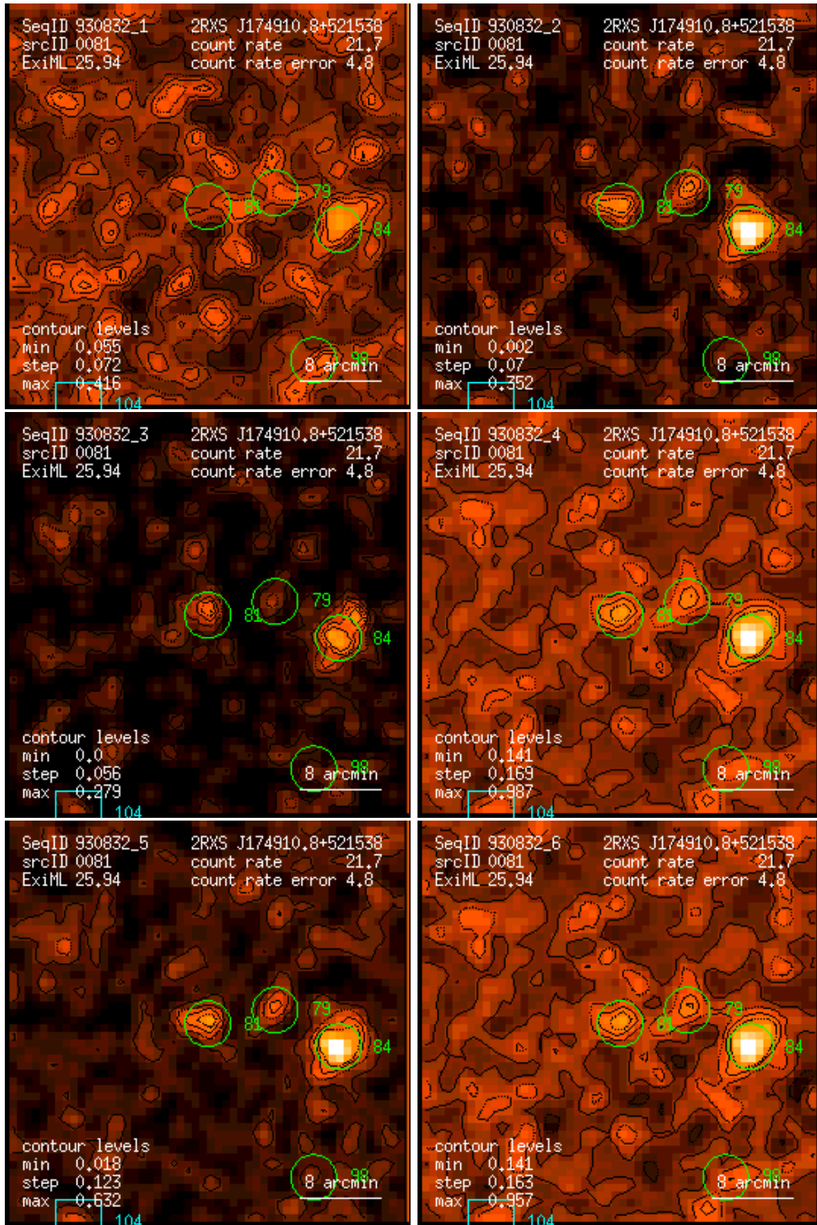
Figure 81: RASS 930832: detection 0081: band rate images, Gaussian filter: (1) PSPC channels 11 – 41, (2) 52 – 90, (3) 91 – 201, (4) 11 – 235, (5) 52 – 201, (6) 11 – 201. Broad band rates in counts/ks. Band rate contour levels in counts/ks/arcmin 2 .
