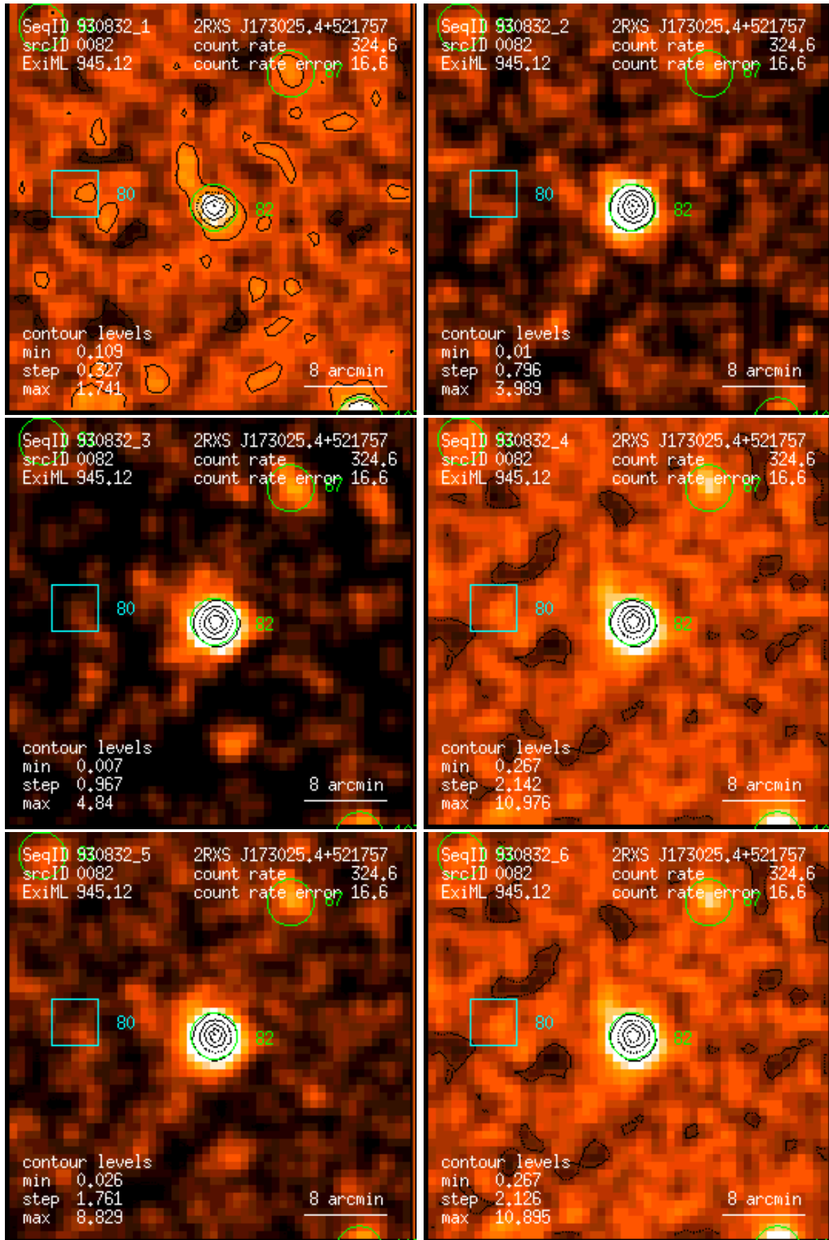
Figure 82: RASS 930832: detection 0082: band rate images, Gaussian filter: (1) PSPC channels 11 – 41, (2) 52 – 90, (3) 91 – 201, (4) 11 – 235, (5) 52 – 201, (6) 11 – 201. Broad band rates in counts/ks. Band rate contour levels in counts/ks/arcmin 2 .
