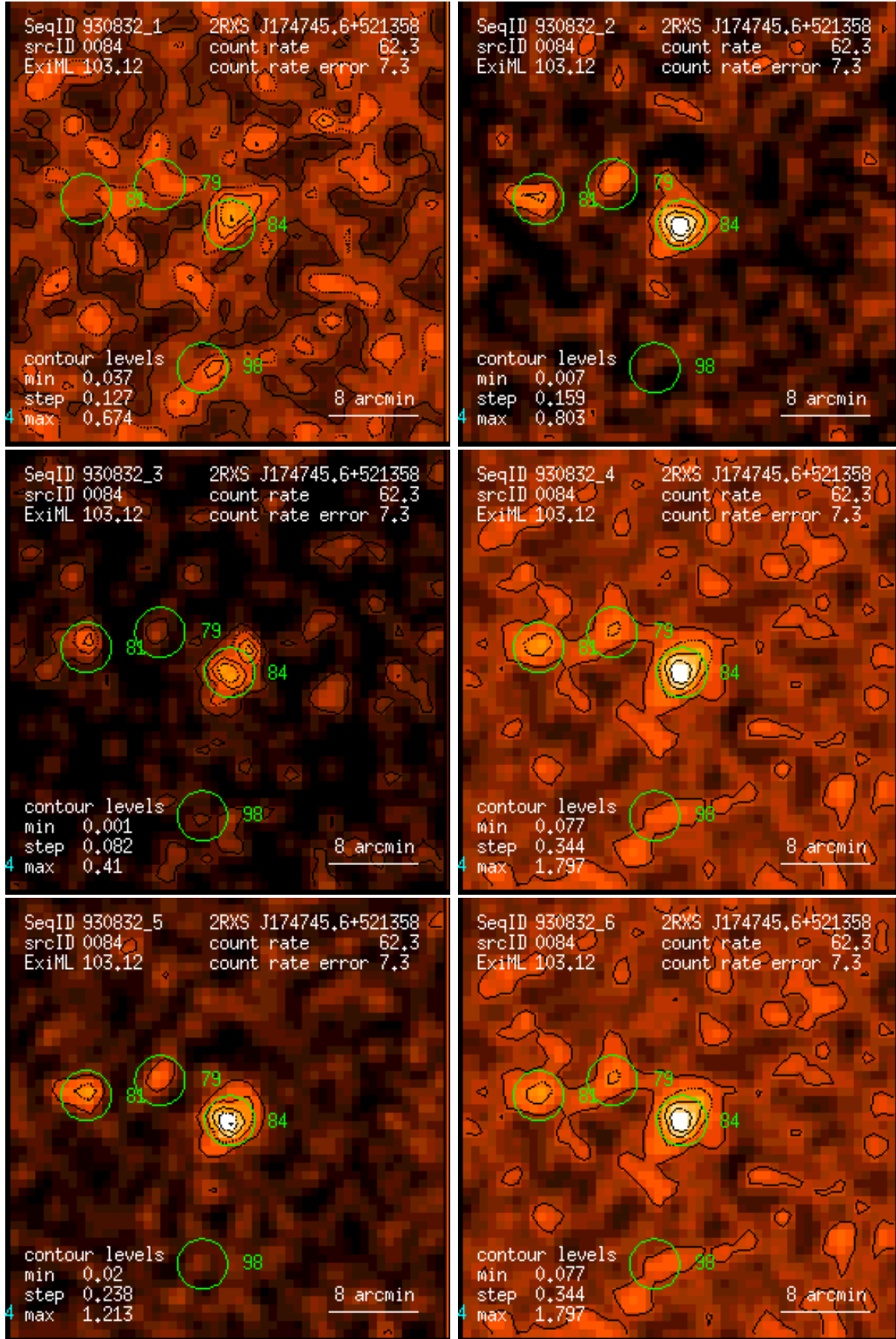
Figure 84: RASS 930832: detection 0084: band rate images, Gaussian filter: (1) PSPC channels 11 – 41, (2) 52 – 90, (3) 91 – 201, (4) 11 – 235, (5) 52 – 201, (6) 11 – 201. Broad band rates in counts/ks. Band rate contour levels in counts/ks/arcmin 2 .
