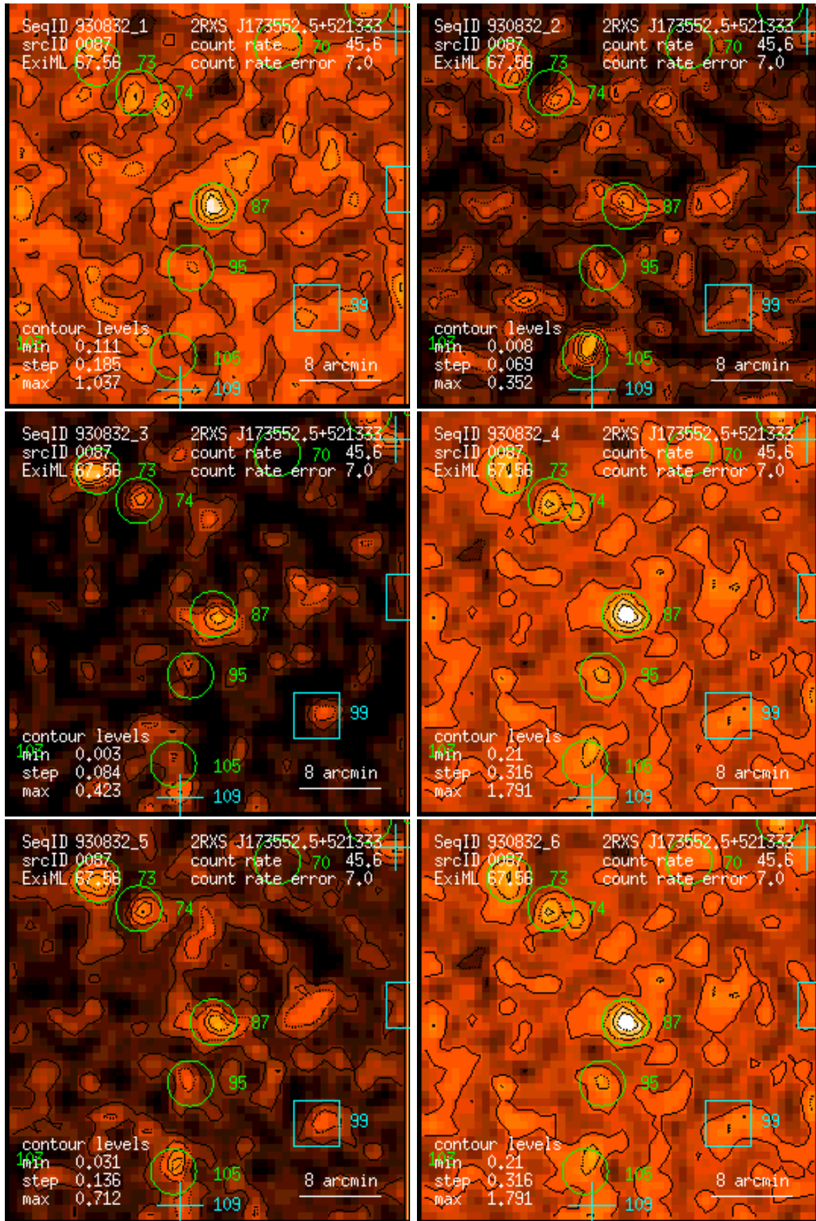
Figure 87: RASS 930832: detection 0087: band rate images, Gaussian filter: (1) PSPC channels 11 – 41, (2) 52 – 90, (3) 91 – 201, (4) 11 – 235, (5) 52 – 201, (6) 11 – 201. Broad band rates in counts/ks. Band rate contour levels in counts/ks/arcmin 2 .
