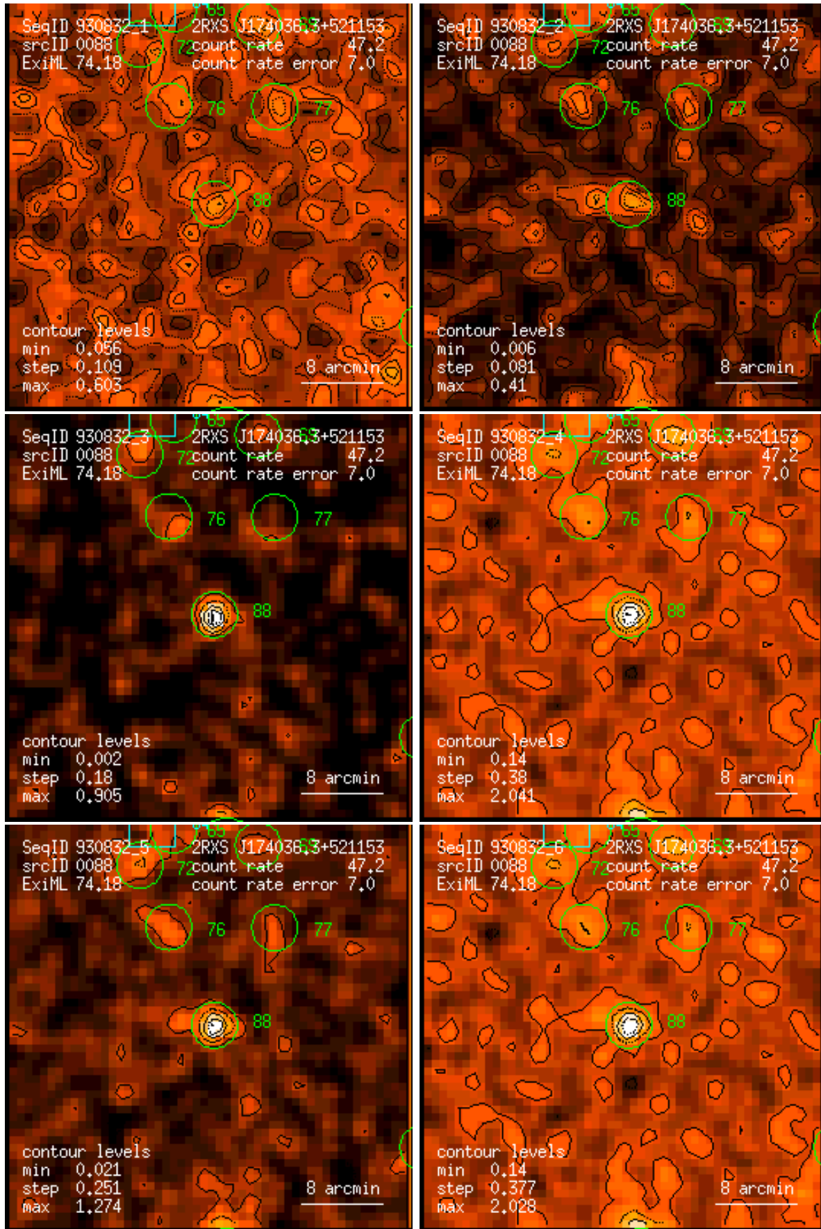
Figure 88: RASS 930832: detection 0088: band rate images, Gaussian filter: (1) PSPC channels 11 – 41, (2) 52 – 90, (3) 91 – 201, (4) 11 – 235, (5) 52 – 201, (6) 11 – 201. Broad band rates in counts/ks. Band rate contour levels in counts/ks/arcmin 2 .
