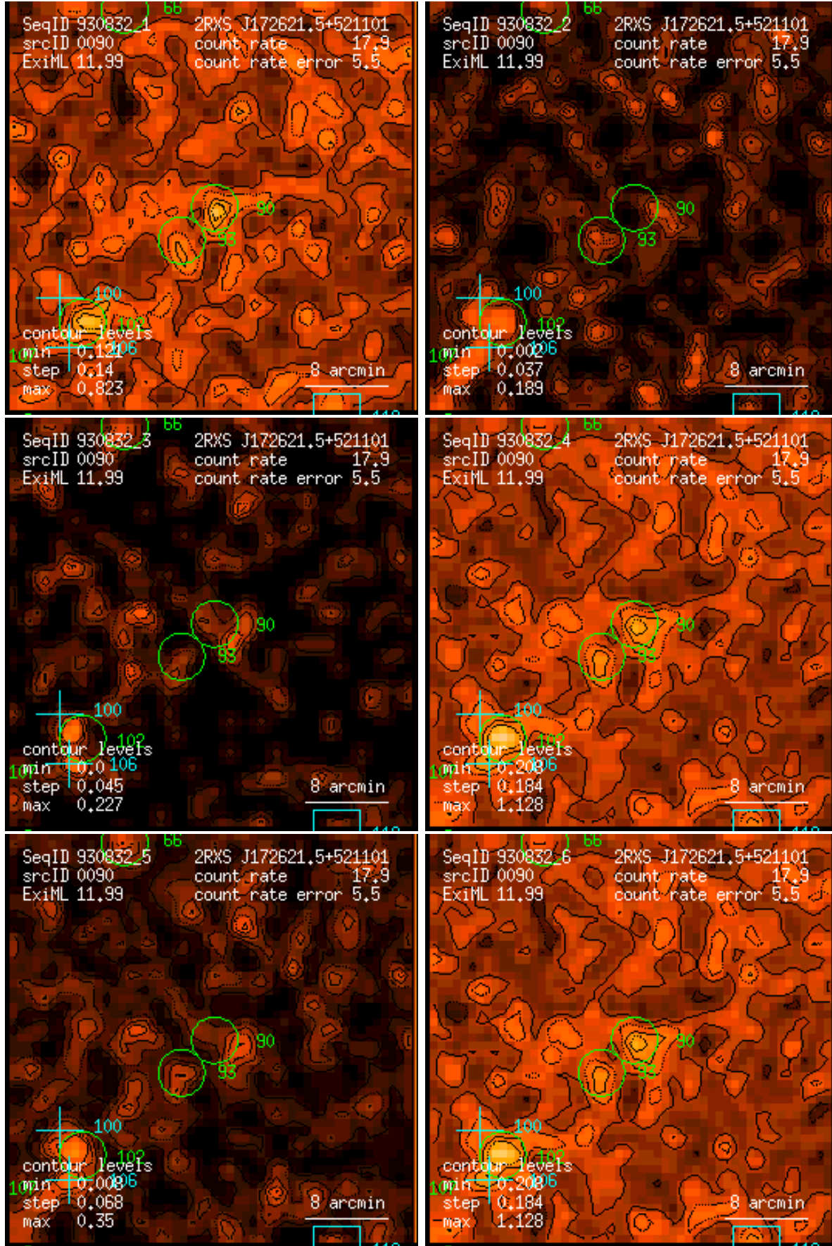
Figure 90: RASS 930832: detection 0090: band rate images, Gaussian filter: (1) PSPC channels 11 – 41, (2) 52 – 90, (3) 91 – 201, (4) 11 – 235, (5) 52 – 201, (6) 11 – 201. Broad band rates in counts/ks. Band rate contour levels in counts/ks/arcmin 2 .
