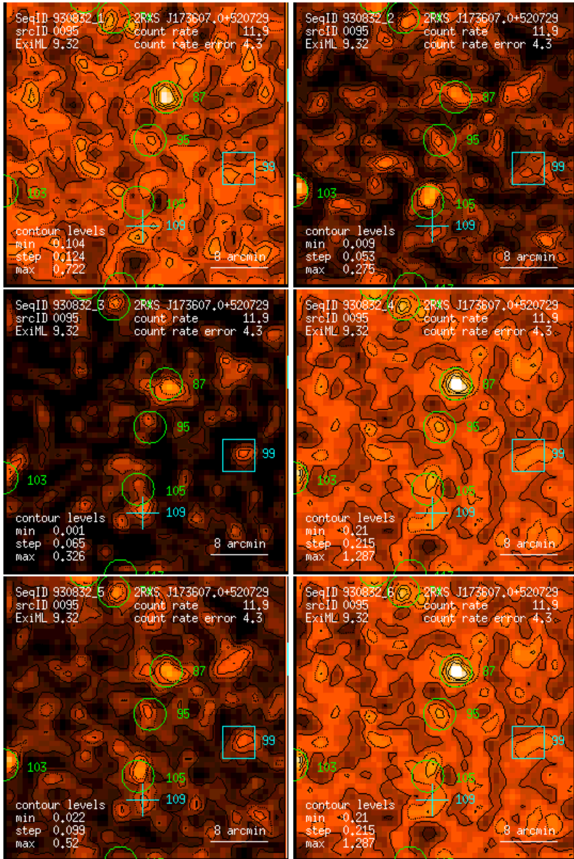
Figure 95: RASS 930832: detection 0095: band rate images, Gaussian filter: (1) PSPC channels 11 – 41, (2) 52 – 90, (3) 91 – 201, (4) 11 – 235, (5) 52 – 201, (6) 11 – 201. Broad band rates in counts/ks. Band rate contour levels in counts/ks/arcmin 2 .
