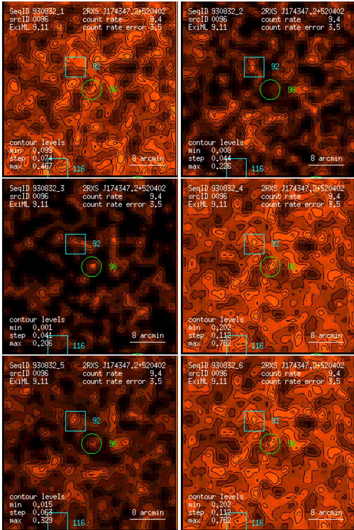
Figure 96: RASS 930832: detection 0096: band rate images, Gaussian filter: (1) PSPC channels 11 – 41, (2) 52 – 90, (3) 91 – 201, (4) 11 – 235, (5) 52 – 201, (6) 11 – 201. Broad band rates in counts/ks. Band rate contour levels in counts/ks/arcmin 2 .
