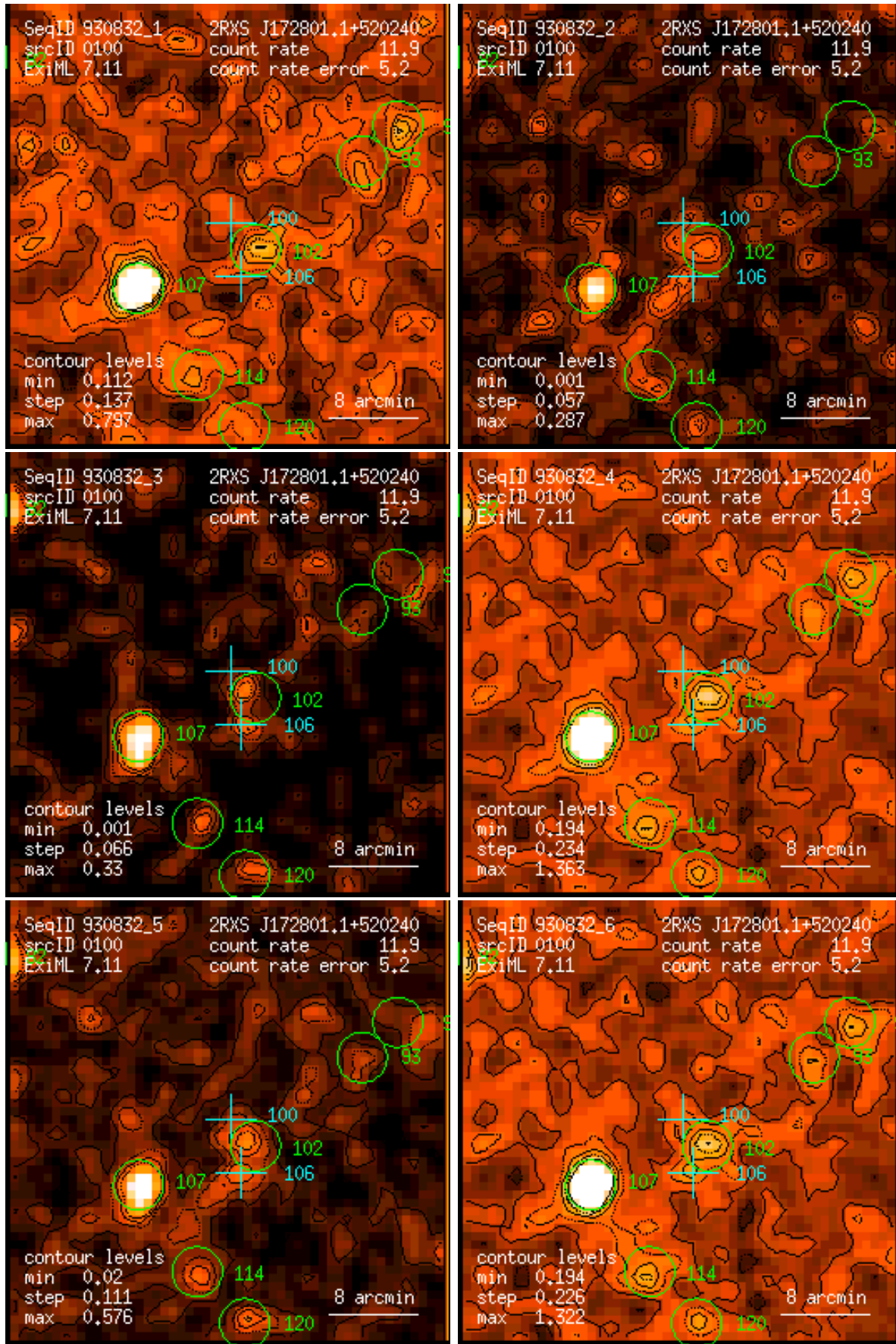
Figure 100: RASS 930832: detection 0100: band rate images, Gaussian filter: (1) PSPC channels 11 – 41, (2) 52 – 90, (3) 91 – 201, (4) 11 – 235, (5) 52 – 201, (6) 11 – 201. Broad band rates in counts/ks. Band rate contour levels in counts/ks/arcmin 2 .
