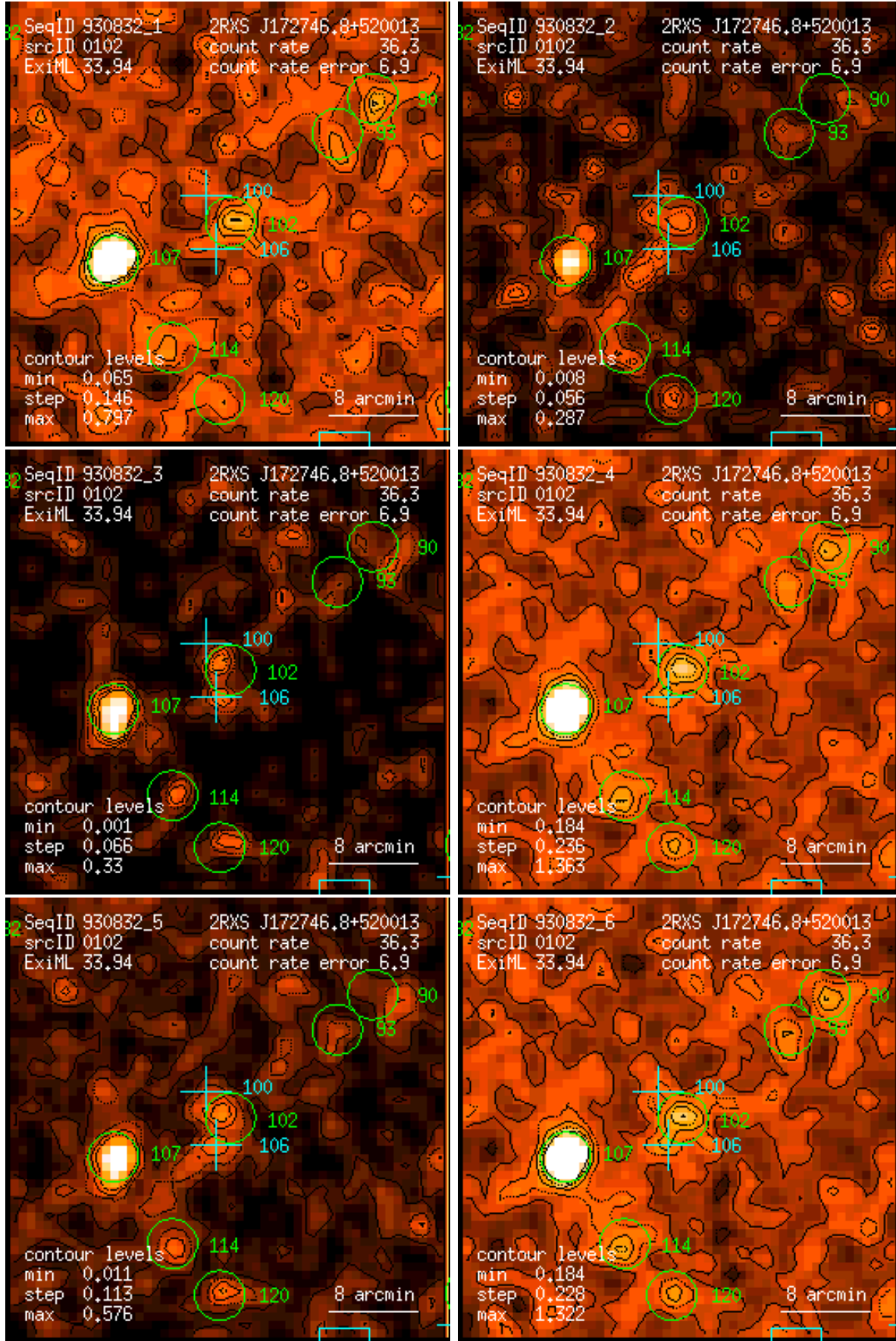
Figure 102: RASS 930832: detection 0102: band rate images, Gaussian filter: (1) PSPC channels 11 – 41, (2) 52 – 90, (3) 91 – 201, (4) 11 – 235, (5) 52 – 201, (6) 11 – 201. Broad band rates in counts/ks. Band rate contour levels in counts/ks/arcmin 2 .
