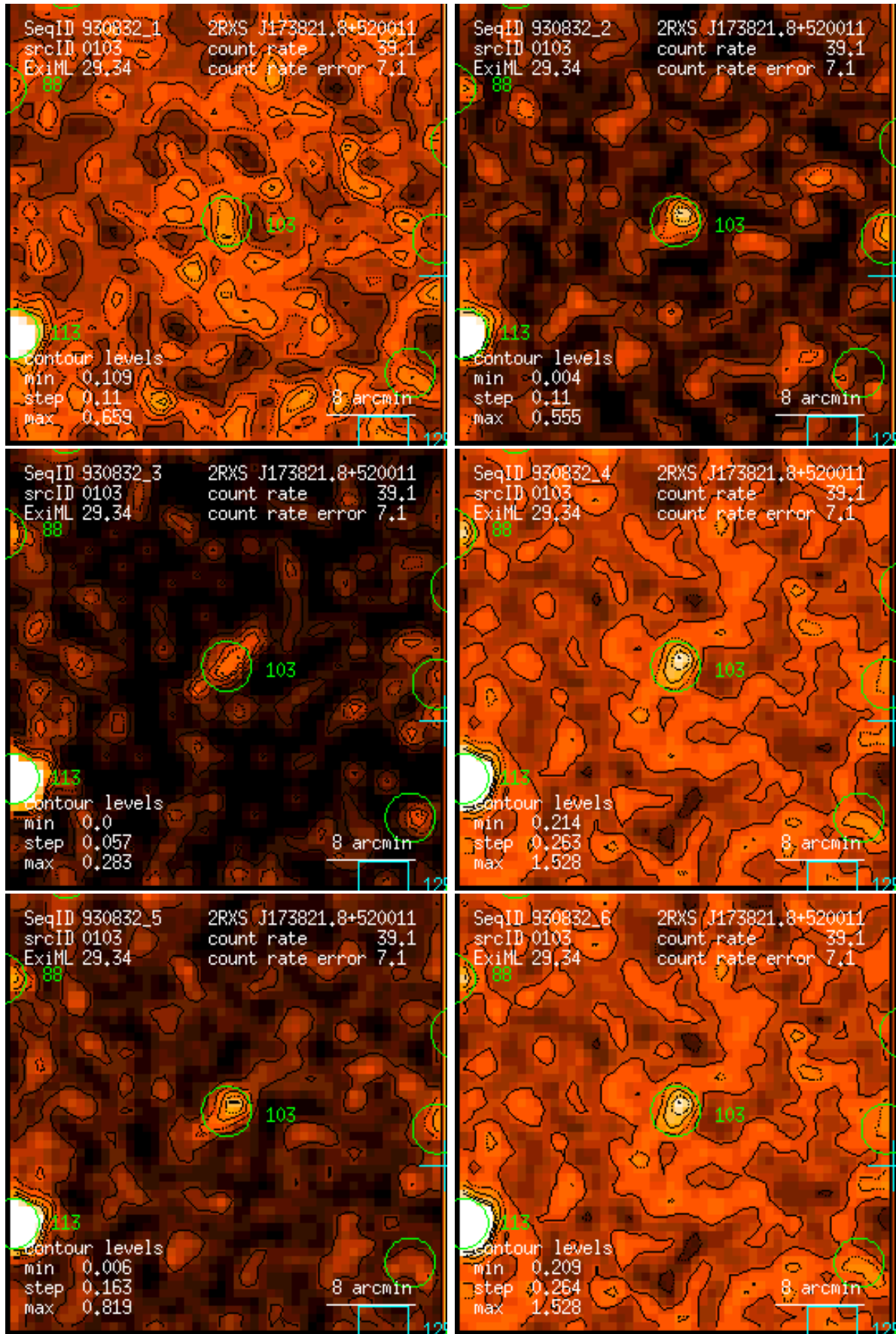
Figure 103: RASS 930832: detection 0103: band rate images, Gaussian filter: (1) PSPC channels 11 – 41, (2) 52 – 90, (3) 91 – 201, (4) 11 – 235, (5) 52 – 201, (6) 11 – 201. Broad band rates in counts/ks. Band rate contour levels in counts/ks/arcmin 2 .
