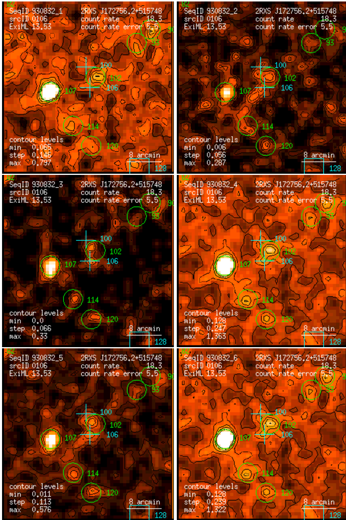
Figure 106: RASS 930832: detection 0106: band rate images, Gaussian filter: (1) PSPC channels 11 – 41, (2) 52 – 90, (3) 91 – 201, (4) 11 – 235, (5) 52 – 201, (6) 11 – 201. Broad band rates in counts/ks. Band rate contour levels in counts/ks/arcmin 2 .
