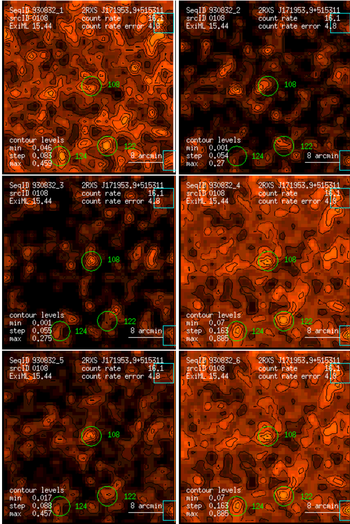
Figure 108: RASS 930832: detection 0108: band rate images, Gaussian filter: (1) PSPC channels 11 – 41, (2) 52 – 90, (3) 91 – 201, (4) 11 – 235, (5) 52 – 201, (6) 11 – 201. Broad band rates in counts/ks. Band rate contour levels in counts/ks/arcmin 2 .
