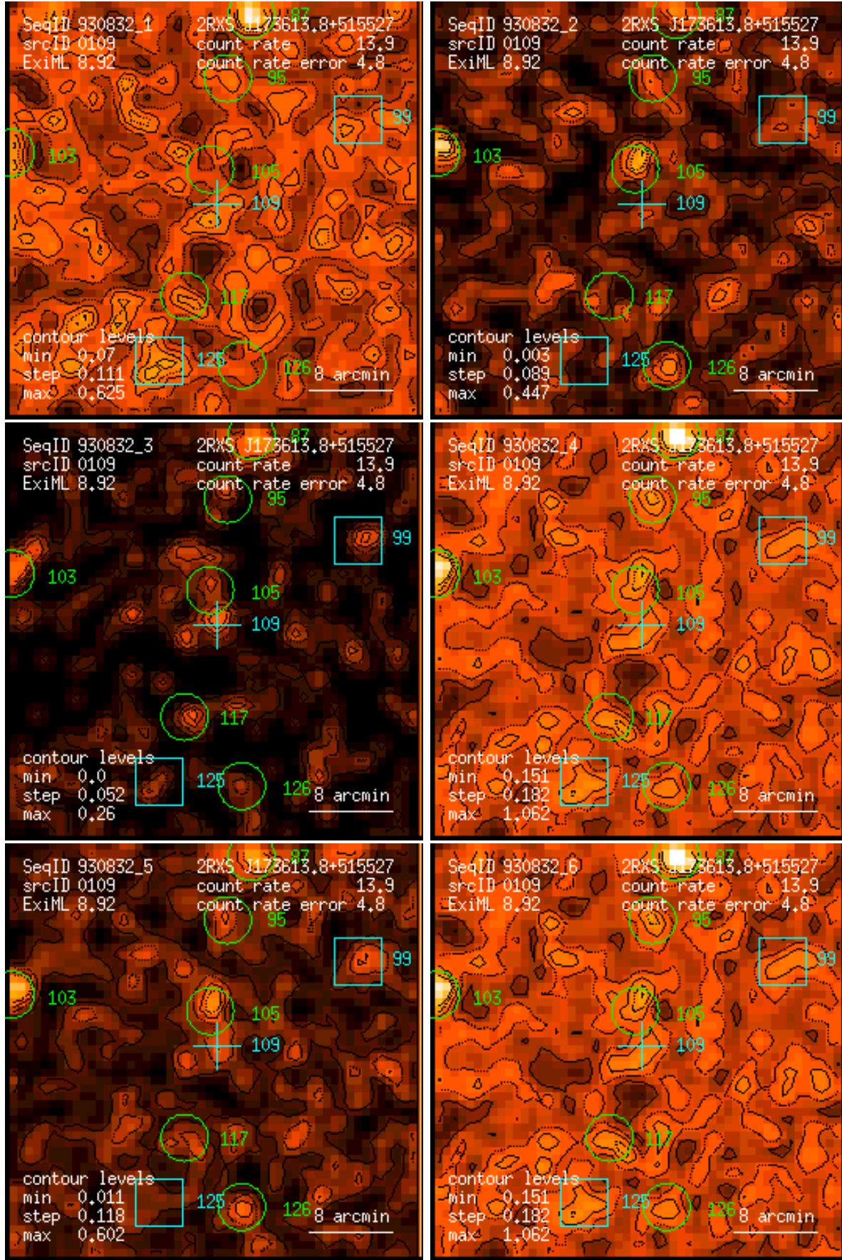
Figure 109: RASS 930832: detection 0109: band rate images, Gaussian filter: (1) PSPC channels 11 – 41, (2) 52 – 90, (3) 91 – 201, (4) 11 – 235, (5) 52 – 201, (6) 11 – 201. Broad band rates in counts/ks. Band rate contour levels in counts/ks/arcmin 2 .
