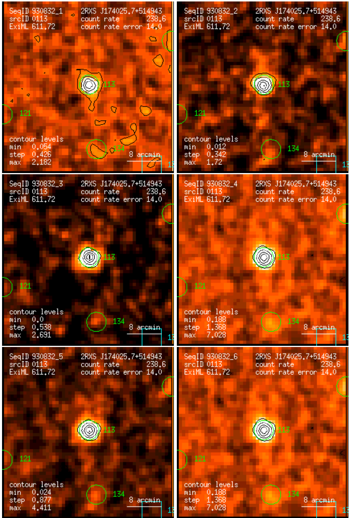
Figure 113: RASS 930832: detection 0113: band rate images, Gaussian filter: (1) PSPC channels 11 – 41, (2) 52 – 90, (3) 91 – 201, (4) 11 – 235, (5) 52 – 201, (6) 11 – 201. Broad band rates in counts/ks. Band rate contour levels in counts/ks/arcmin 2 .
