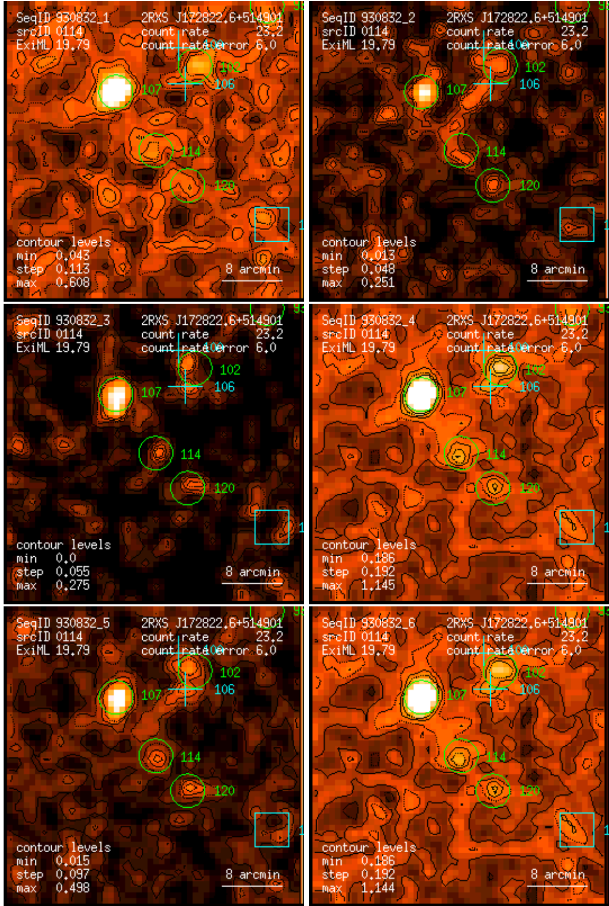
Figure 114: RASS 930832: detection 0114: band rate images, Gaussian filter: (1) PSPC channels 11 – 41, (2) 52 – 90, (3) 91 – 201, (4) 11 – 235, (5) 52 – 201, (6) 11 – 201. Broad band rates in counts/ks. Band rate contour levels in counts/ks/arcmin 2 .
