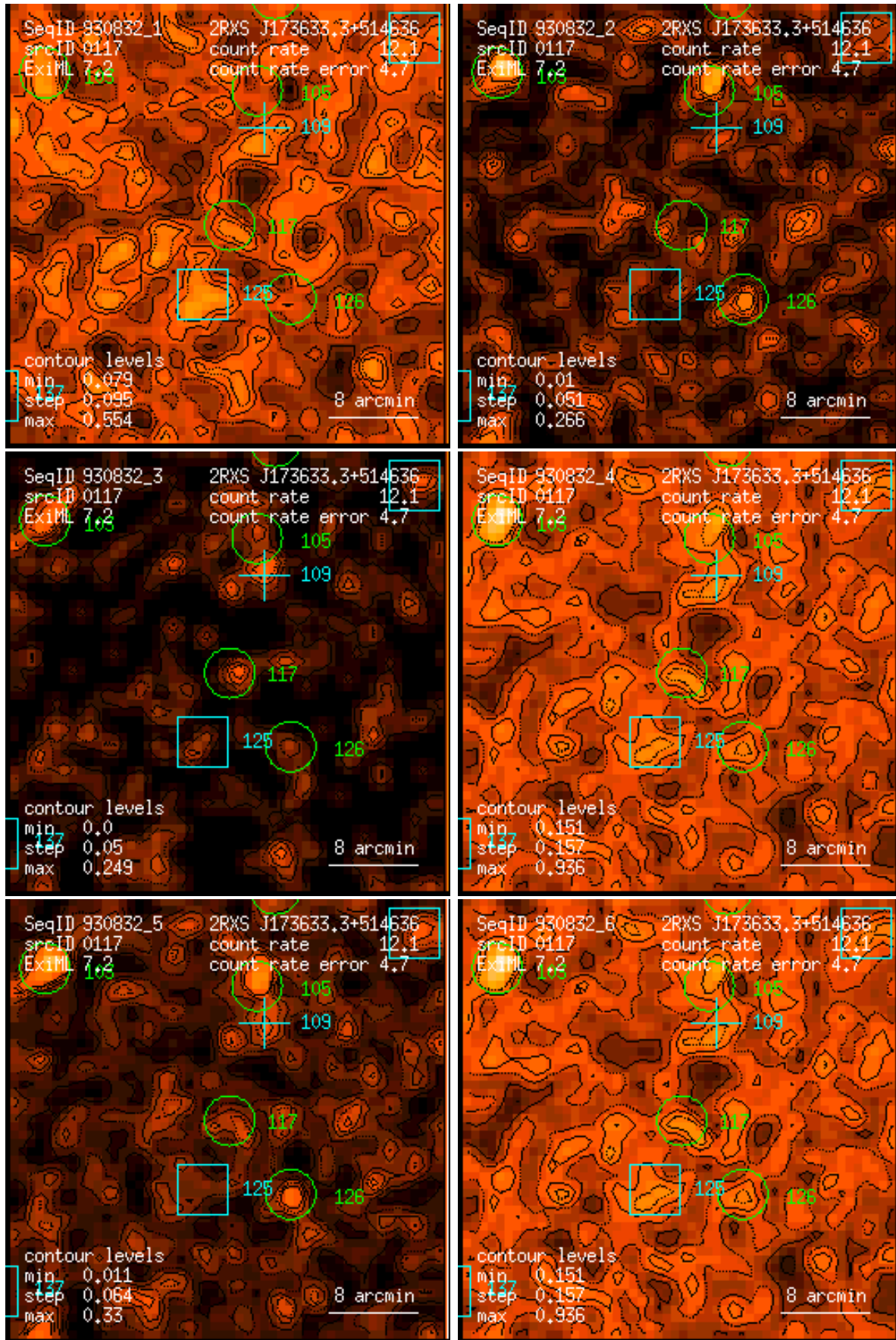
Figure 117: RASS 930832: detection 0117: band rate images, Gaussian filter: (1) PSPC channels 11 – 41, (2) 52 – 90, (3) 91 – 201, (4) 11 – 235, (5) 52 – 201, (6) 11 – 201. Broad band rates in counts/ks. Band rate contour levels in counts/ks/arcmin 2 .
