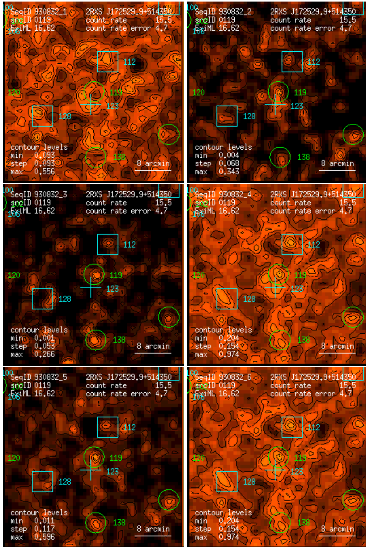
Figure 119: RASS 930832: detection 0119: band rate images, Gaussian filter: (1) PSPC channels 11 – 41, (2) 52 – 90, (3) 91 – 201, (4) 11 – 235, (5) 52 – 201, (6) 11 – 201. Broad band rates in counts/ks. Band rate contour levels in counts/ks/arcmin 2 .
