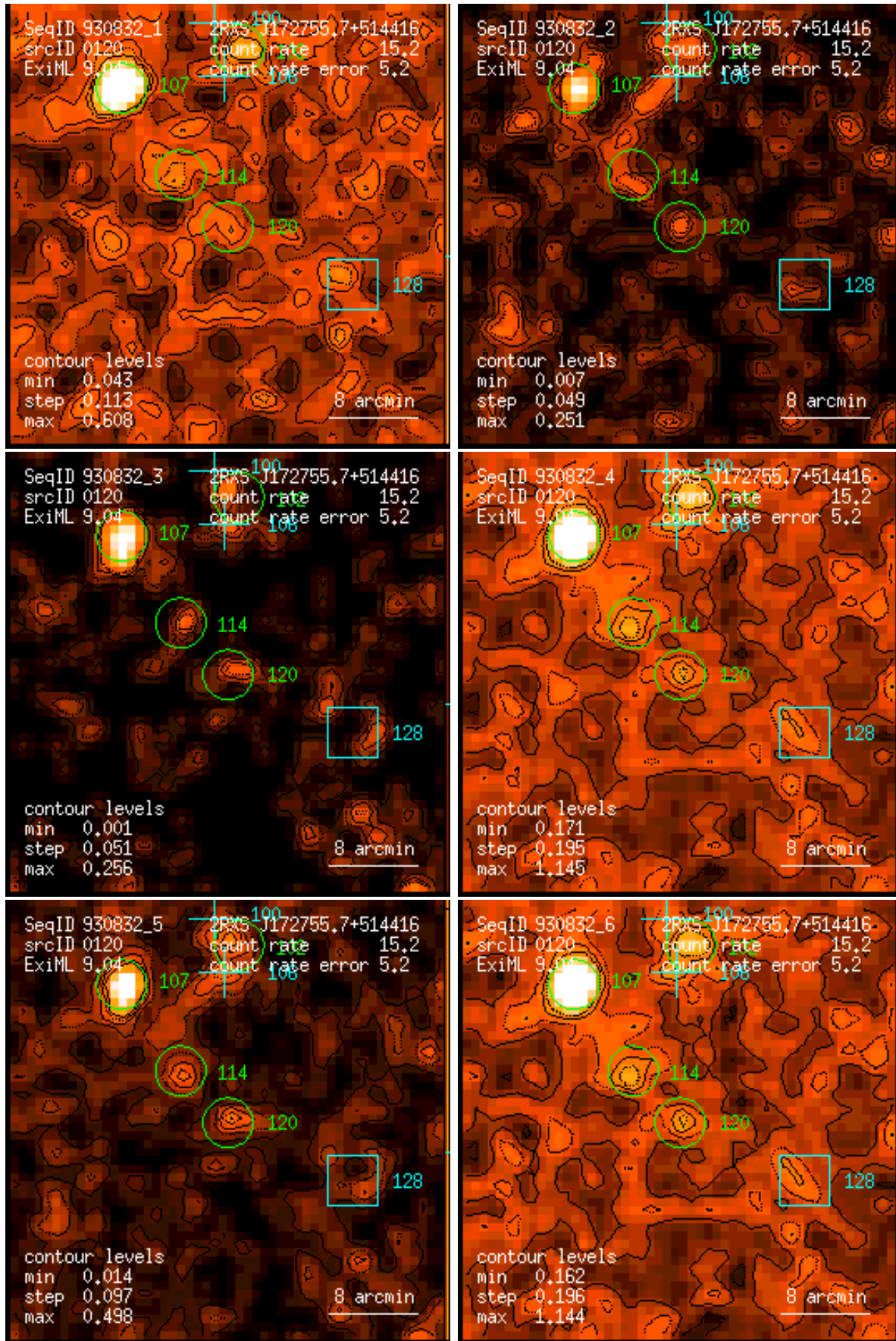
Figure 120: RASS 930832: detection 0120: band rate images, Gaussian filter: (1) PSPC channels 11 – 41, (2) 52 – 90, (3) 91 – 201, (4) 11 – 235, (5) 52 – 201, (6) 11 – 201. Broad band rates in counts/ks. Band rate contour levels in counts/ks/arcmin 2 .
