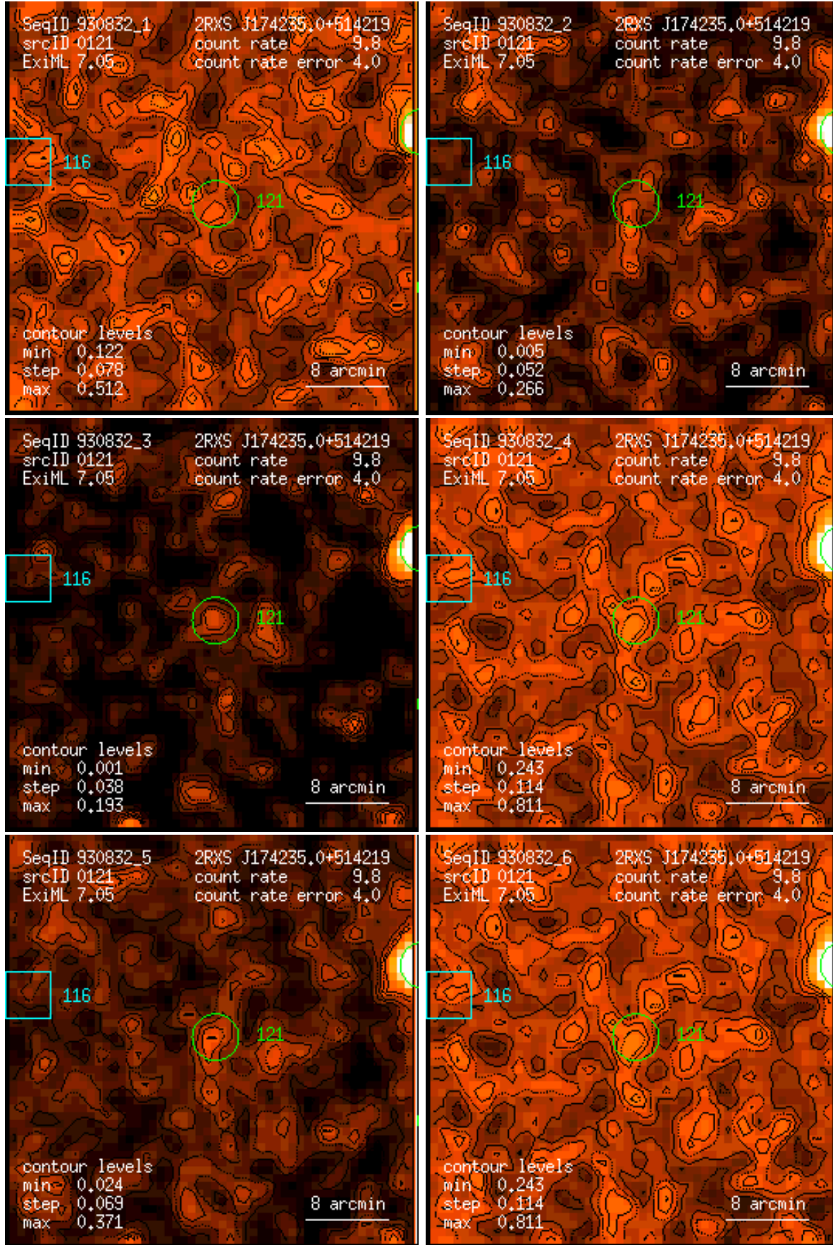
Figure 121: RASS 930832: detection 0121: band rate images, Gaussian filter: (1) PSPC channels 11 – 41, (2) 52 – 90, (3) 91 – 201, (4) 11 – 235, (5) 52 – 201, (6) 11 – 201. Broad band rates in counts/ks. Band rate contour levels in counts/ks/arcmin 2 .
