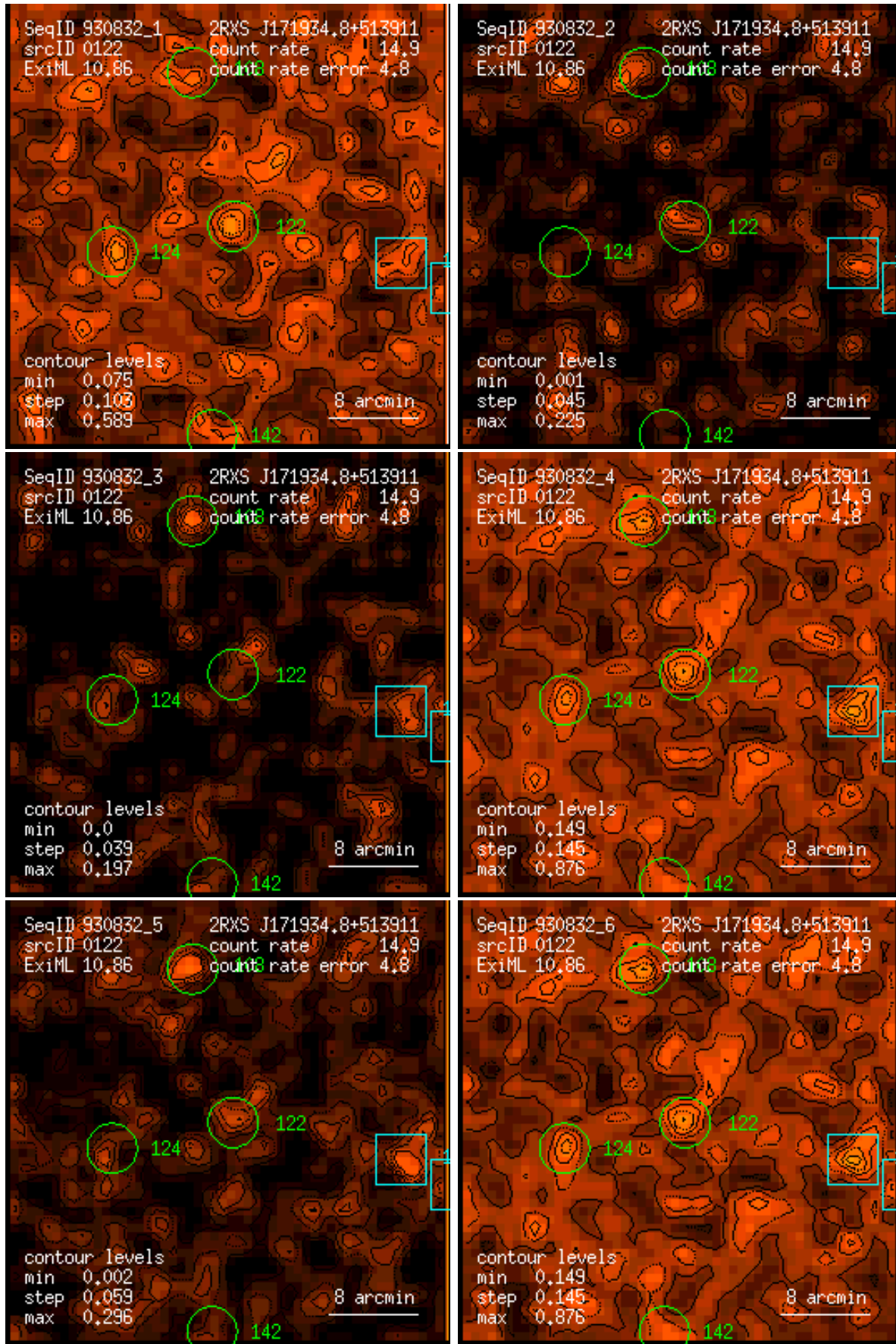
Figure 122: RASS 930832: detection 0122: band rate images, Gaussian filter: (1) PSPC channels 11 – 41, (2) 52 – 90, (3) 91 – 201, (4) 11 – 235, (5) 52 – 201, (6) 11 – 201. Broad band rates in counts/ks. Band rate contour levels in counts/ks/arcmin 2 .
