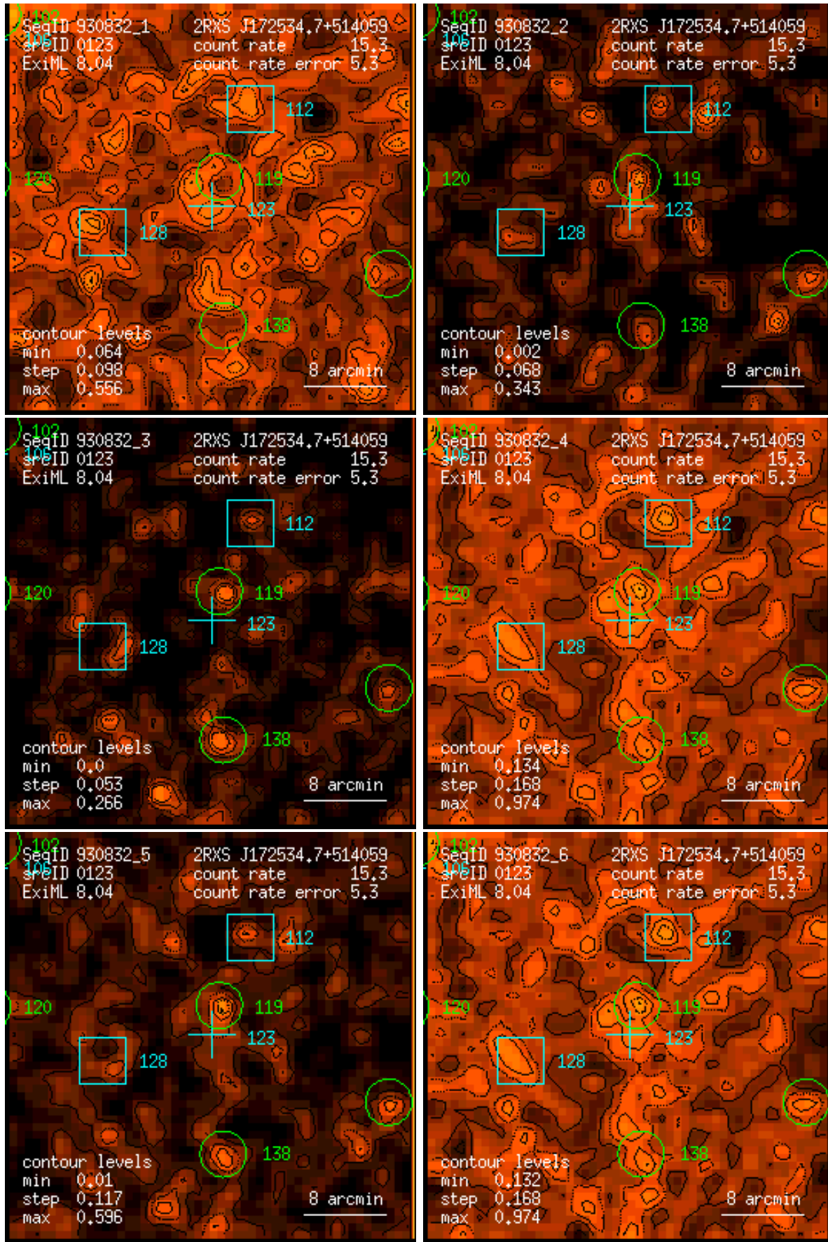
Figure 123: RASS 930832: detection 0123: band rate images, Gaussian filter: (1) PSPC channels 11 – 41, (2) 52 – 90, (3) 91 – 201, (4) 11 – 235, (5) 52 – 201, (6) 11 – 201. Broad band rates in counts/ks. Band rate contour levels in counts/ks/arcmin 2 .
