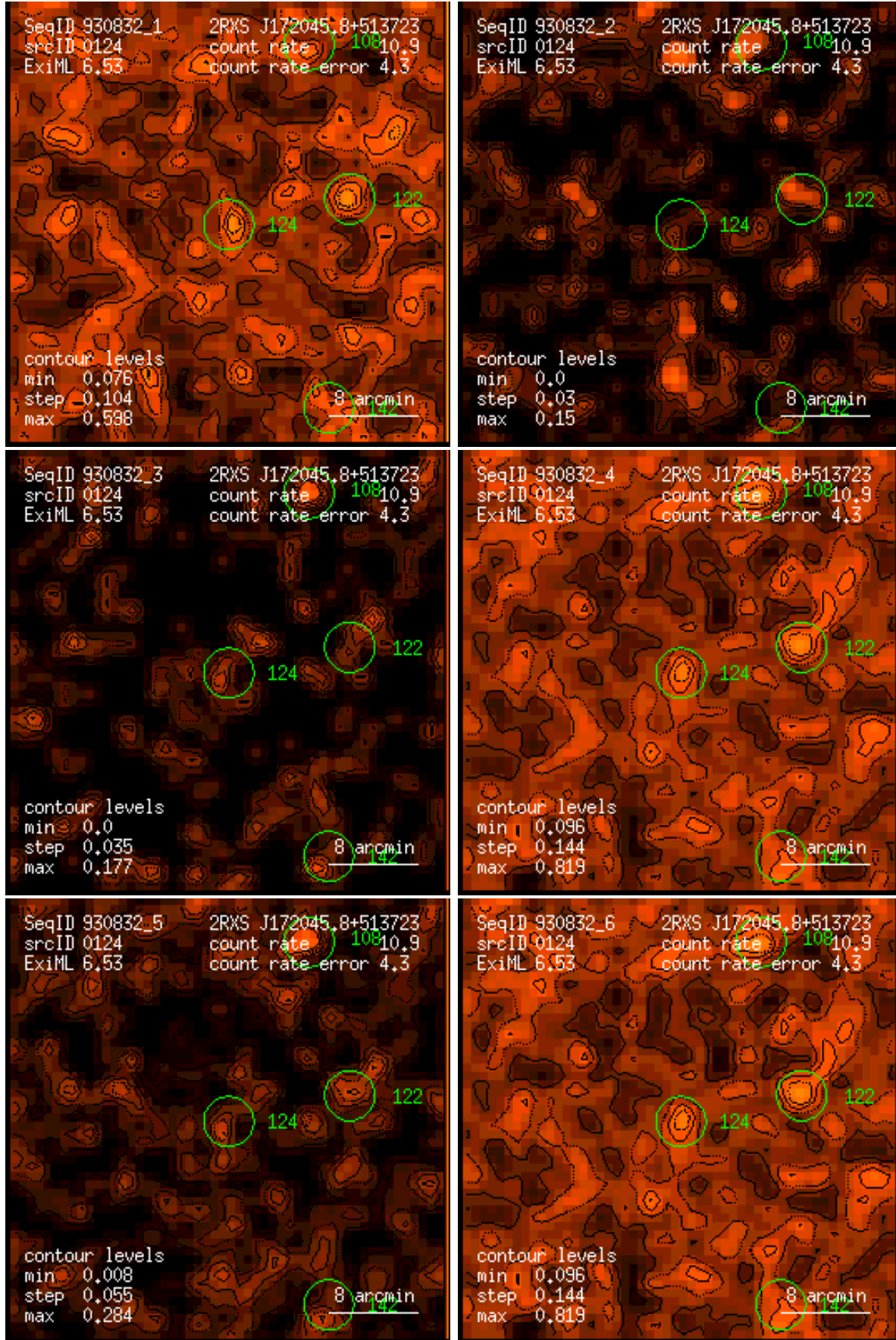
Figure 124: RASS 930832: detection 0124: band rate images, Gaussian filter: (1) PSPC channels 11 – 41, (2) 52 – 90, (3) 91 – 201, (4) 11 – 235, (5) 52 – 201, (6) 11 – 201. Broad band rates in counts/ks. Band rate contour levels in counts/ks/arcmin 2 .
