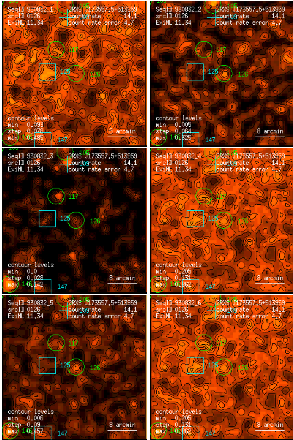
Figure 126: RASS 930832: detection 0126: band rate images, Gaussian filter: (1) PSPC channels 11 – 41, (2) 52 – 90, (3) 91 – 201, (4) 11 – 235, (5) 52 – 201, (6) 11 – 201. Broad band rates in counts/ks. Band rate contour levels in counts/ks/arcmin 2 .
