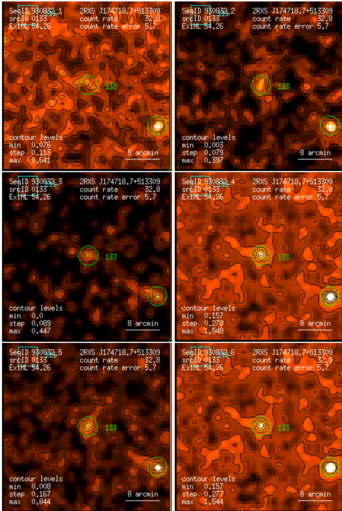
Figure 133: RASS 930832: detection 0133: band rate images, Gaussian filter: (1) PSPC channels 11 – 41, (2) 52 – 90, (3) 91 – 201, (4) 11 – 235, (5) 52 – 201, (6) 11 – 201. Broad band rates in counts/ks. Band rate contour levels in counts/ks/arcmin 2 .
