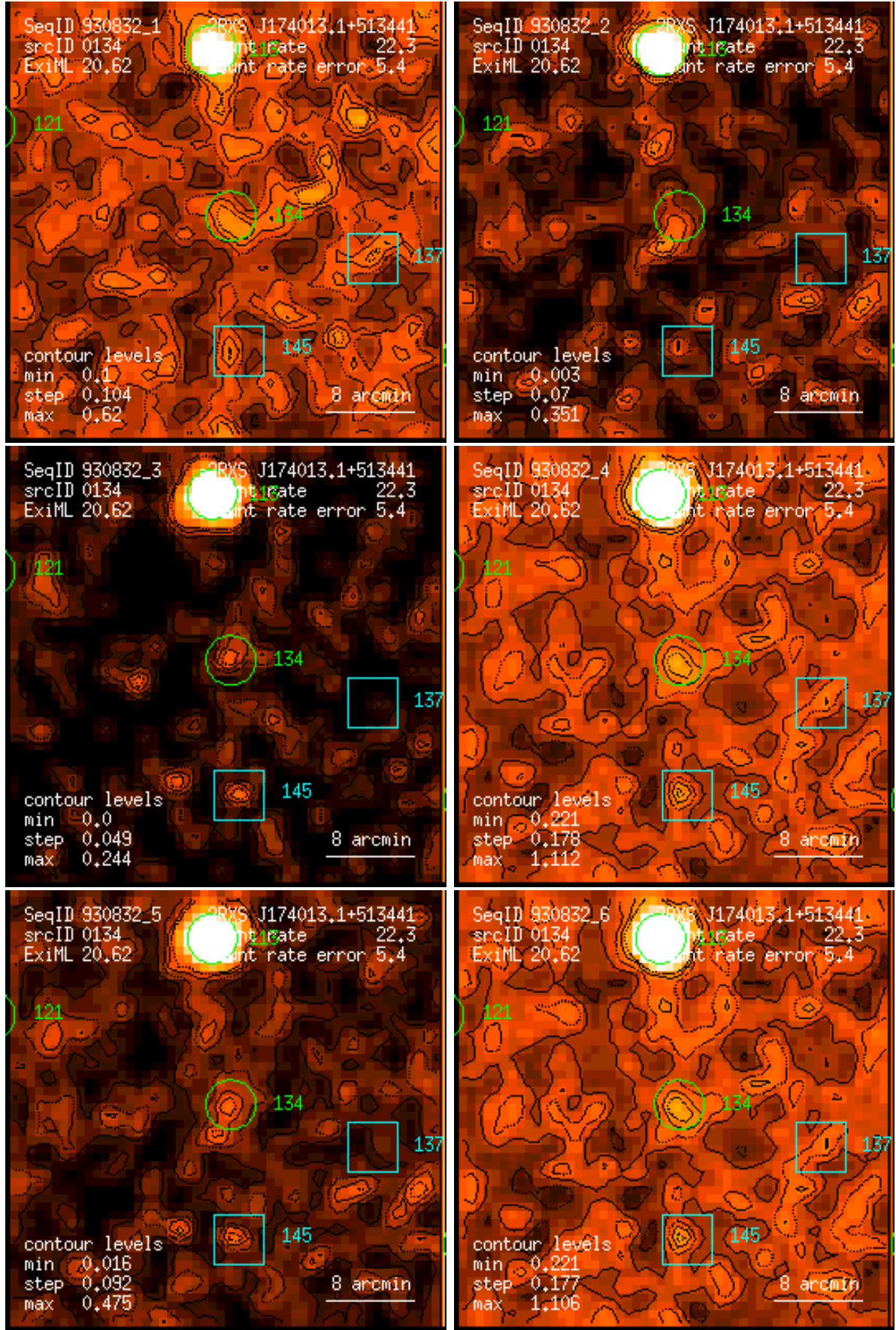
Figure 134: RASS 930832: detection 0134: band rate images, Gaussian filter: (1) PSPC channels 11 – 41, (2) 52 – 90, (3) 91 – 201, (4) 11 – 235, (5) 52 – 201, (6) 11 – 201. Broad band rates in counts/ks. Band rate contour levels in counts/ks/arcmin 2 .
