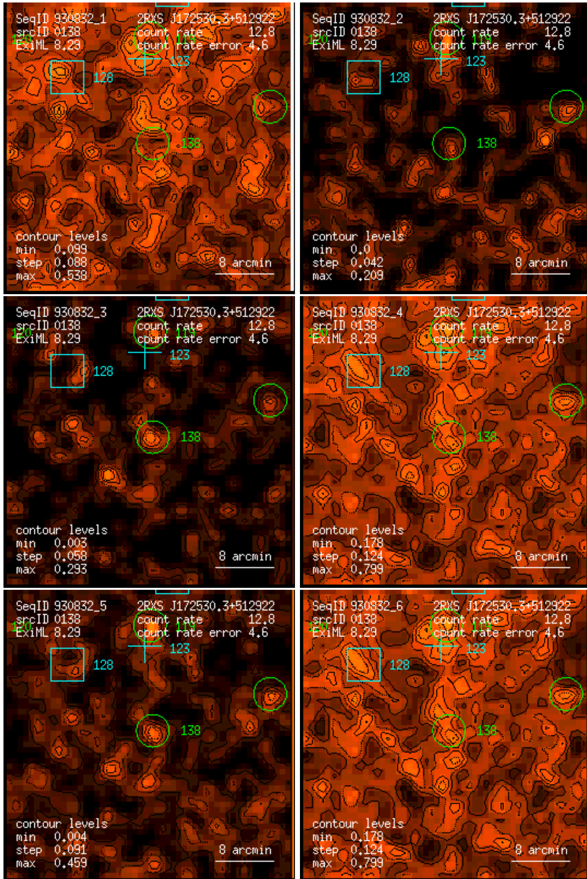
Figure 138: RASS 930832: detection 0138: band rate images, Gaussian filter: (1) PSPC channels 11 – 41, (2) 52 – 90, (3) 91 – 201, (4) 11 – 235, (5) 52 – 201, (6) 11 – 201. Broad band rates in counts/ks. Band rate contour levels in counts/ks/arcmin 2 .
