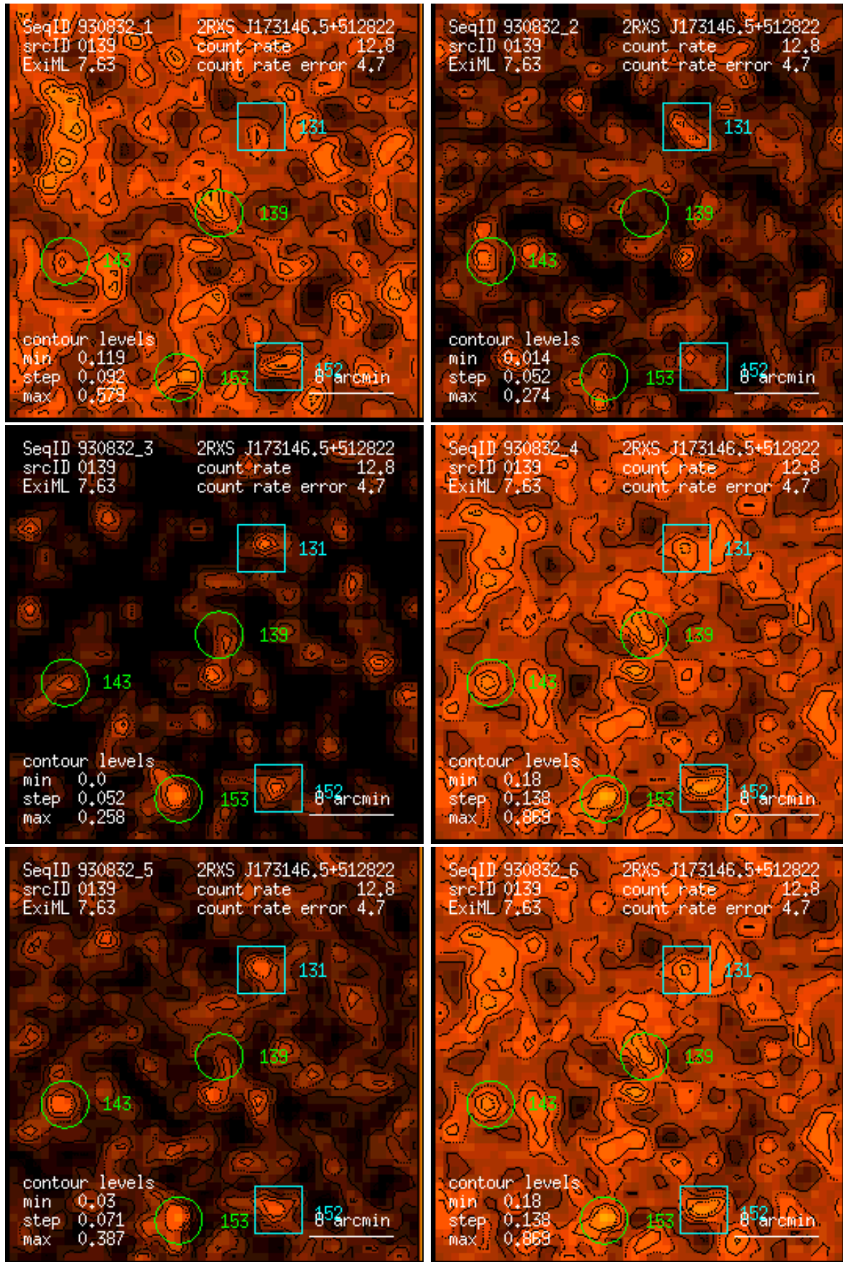
Figure 139: RASS 930832: detection 0139: band rate images, Gaussian filter: (1) PSPC channels 11 – 41, (2) 52 – 90, (3) 91 – 201, (4) 11 – 235, (5) 52 – 201, (6) 11 – 201. Broad band rates in counts/ks. Band rate contour levels in counts/ks/arcmin 2 .
